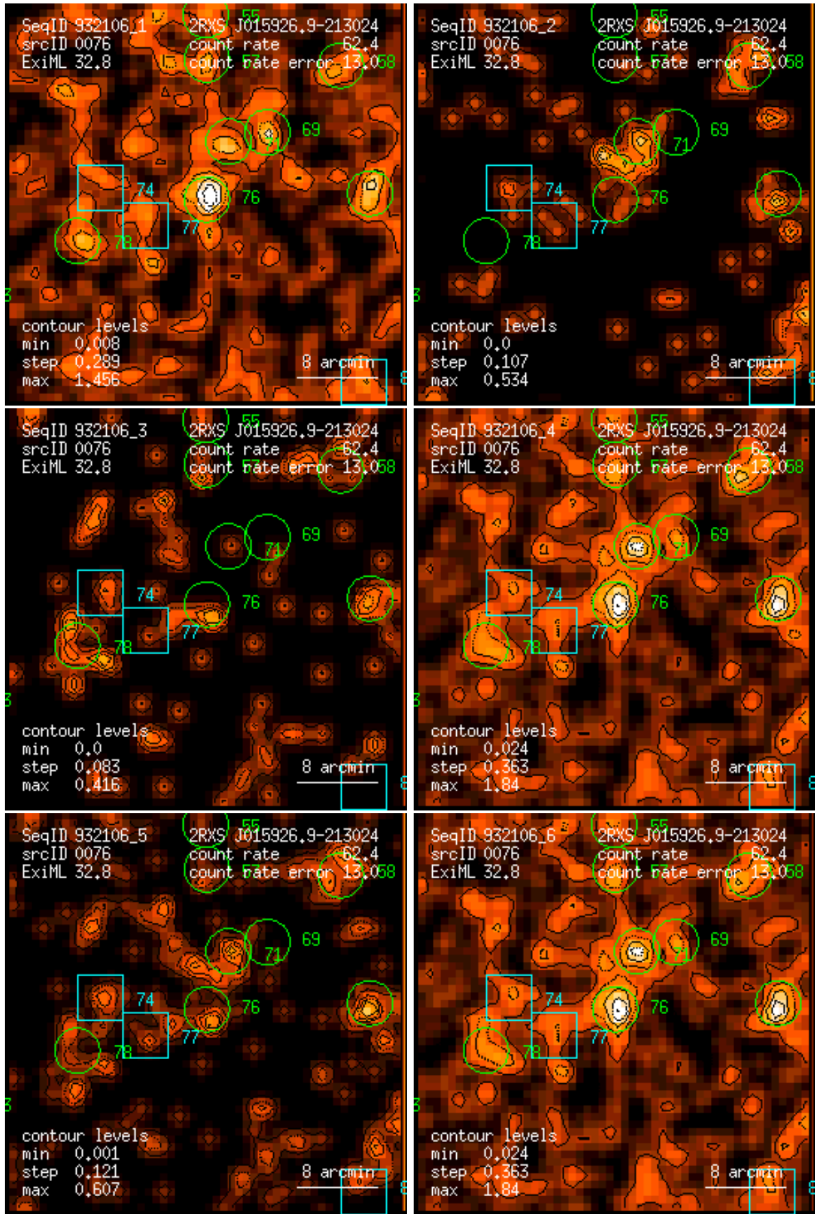
Figure 76: RASS 932106: detection 0076: band rate images, Gaussian filter: (1) PSPC channels 11 – 41, (2) 52 – 90, (3) 91 – 201, (4) 11 – 235, (5) 52 – 201, (6) 11 – 201. Broad band rates in counts/ks. Band rate contour levels in counts/ks/arcmin 2 .
