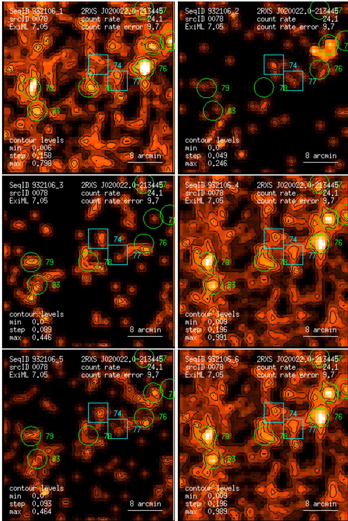
Figure 78: RASS 932106: detection 0078: band rate images, Gaussian filter: (1) PSPC channels 11 – 41, (2) 52 – 90, (3) 91 – 201, (4) 11 – 235, (5) 52 – 201, (6) 11 – 201. Broad band rates in counts/ks. Band rate contour levels in counts/ks/arcmin 2 .
