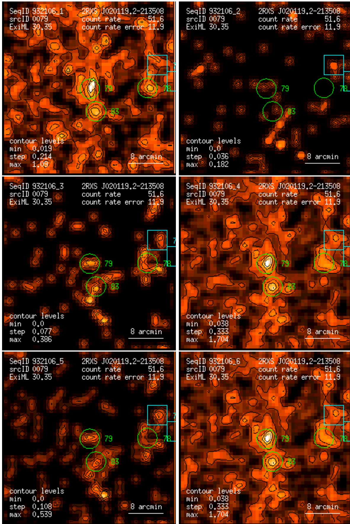
Figure 79: RASS 932106: detection 0079: band rate images, Gaussian filter: (1) PSPC channels 11 – 41, (2) 52 – 90, (3) 91 – 201, (4) 11 – 235, (5) 52 – 201, (6) 11 – 201. Broad band rates in counts/ks. Band rate contour levels in counts/ks/arcmin 2 .
