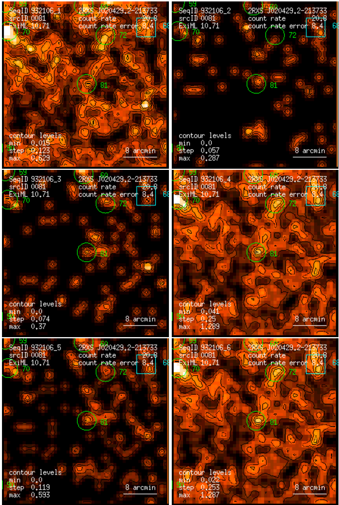
Figure 81: RASS 932106: detection 0081: band rate images, Gaussian filter: (1) PSPC channels 11 – 41, (2) 52 – 90, (3) 91 – 201, (4) 11 – 235, (5) 52 – 201, (6) 11 – 201. Broad band rates in counts/ks. Band rate contour levels in counts/ks/arcmin 2 .
