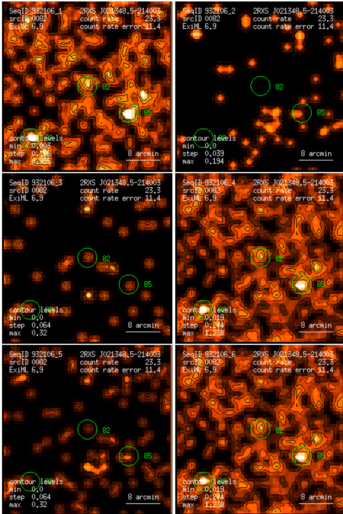
Figure 82: RASS 932106: detection 0082: band rate images, Gaussian filter: (1) PSPC channels 11 – 41, (2) 52 – 90, (3) 91 – 201, (4) 11 – 235, (5) 52 – 201, (6) 11 – 201. Broad band rates in counts/ks. Band rate contour levels in counts/ks/arcmin 2 .
