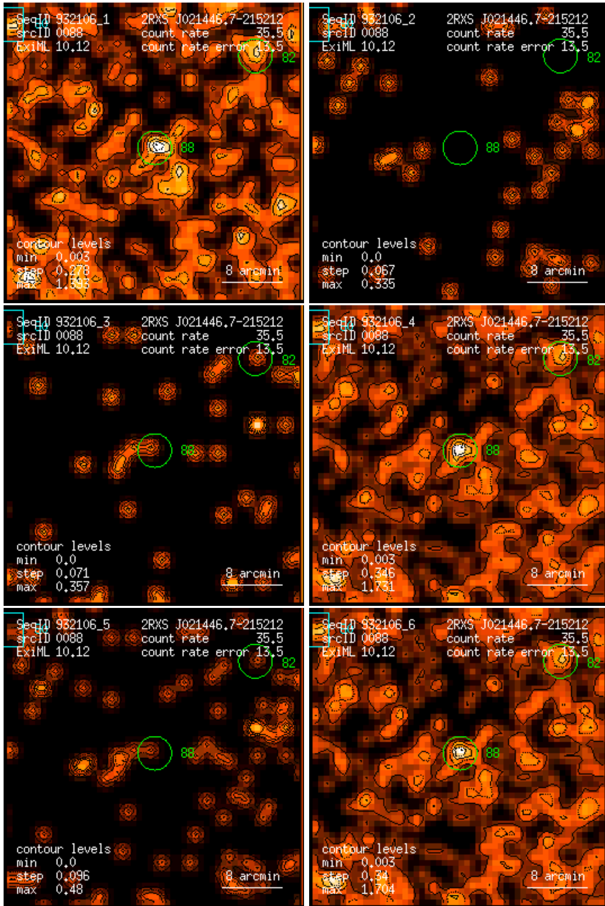
Figure 88: RASS 932106: detection 0088: band rate images, Gaussian filter: (1) PSPC channels 11 – 41, (2) 52 – 90, (3) 91 – 201, (4) 11 – 235, (5) 52 – 201, (6) 11 – 201. Broad band rates in counts/ks. Band rate contour levels in counts/ks/arcmin 2 .
