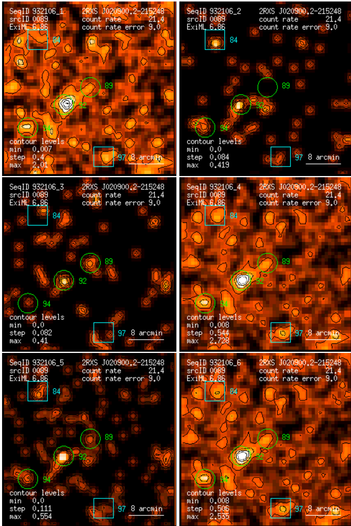
Figure 89: RASS 932106: detection 0089: band rate images, Gaussian filter: (1) PSPC channels 11 – 41, (2) 52 – 90, (3) 91 – 201, (4) 11 – 235, (5) 52 – 201, (6) 11 – 201. Broad band rates in counts/ks. Band rate contour levels in counts/ks/arcmin 2 .
