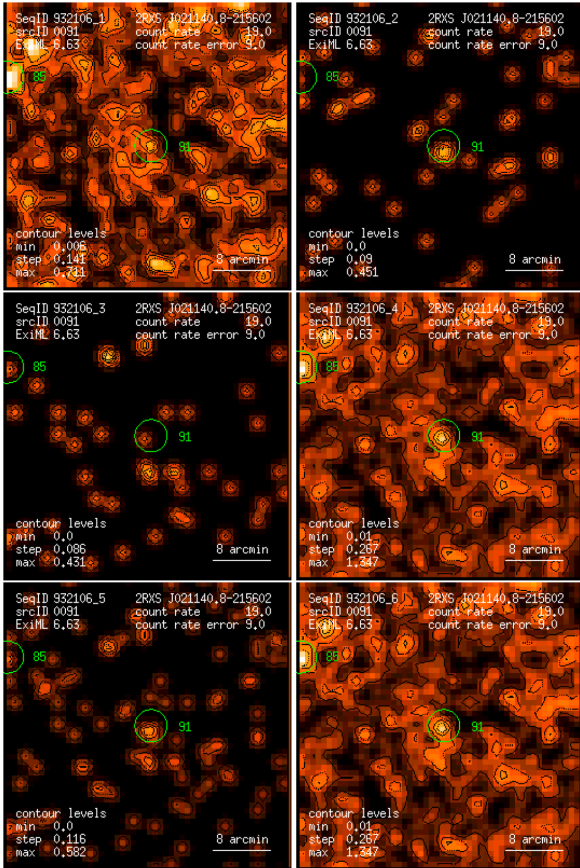
Figure 91: RASS 932106: detection 0091: band rate images, Gaussian filter: (1) PSPC channels 11 – 41, (2) 52 – 90, (3) 91 – 201, (4) 11 – 235, (5) 52 – 201, (6) 11 – 201. Broad band rates in counts/ks. Band rate contour levels in counts/ks/arcmin 2 .
