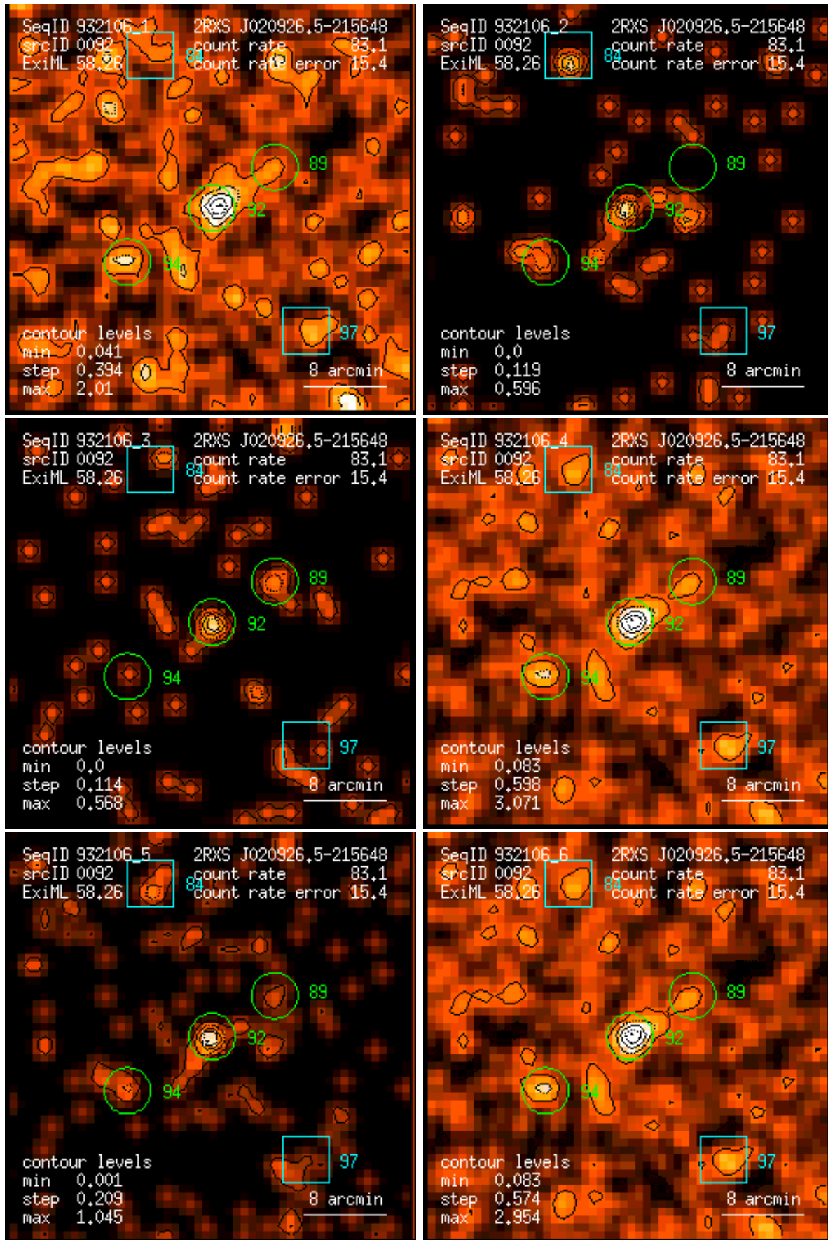
Figure 92: RASS 932106: detection 0092: band rate images, Gaussian filter: (1) PSPC channels 11 – 41, (2) 52 – 90, (3) 91 – 201, (4) 11 – 235, (5) 52 – 201, (6) 11 – 201. Broad band rates in counts/ks. Band rate contour levels in counts/ks/arcmin 2 .
