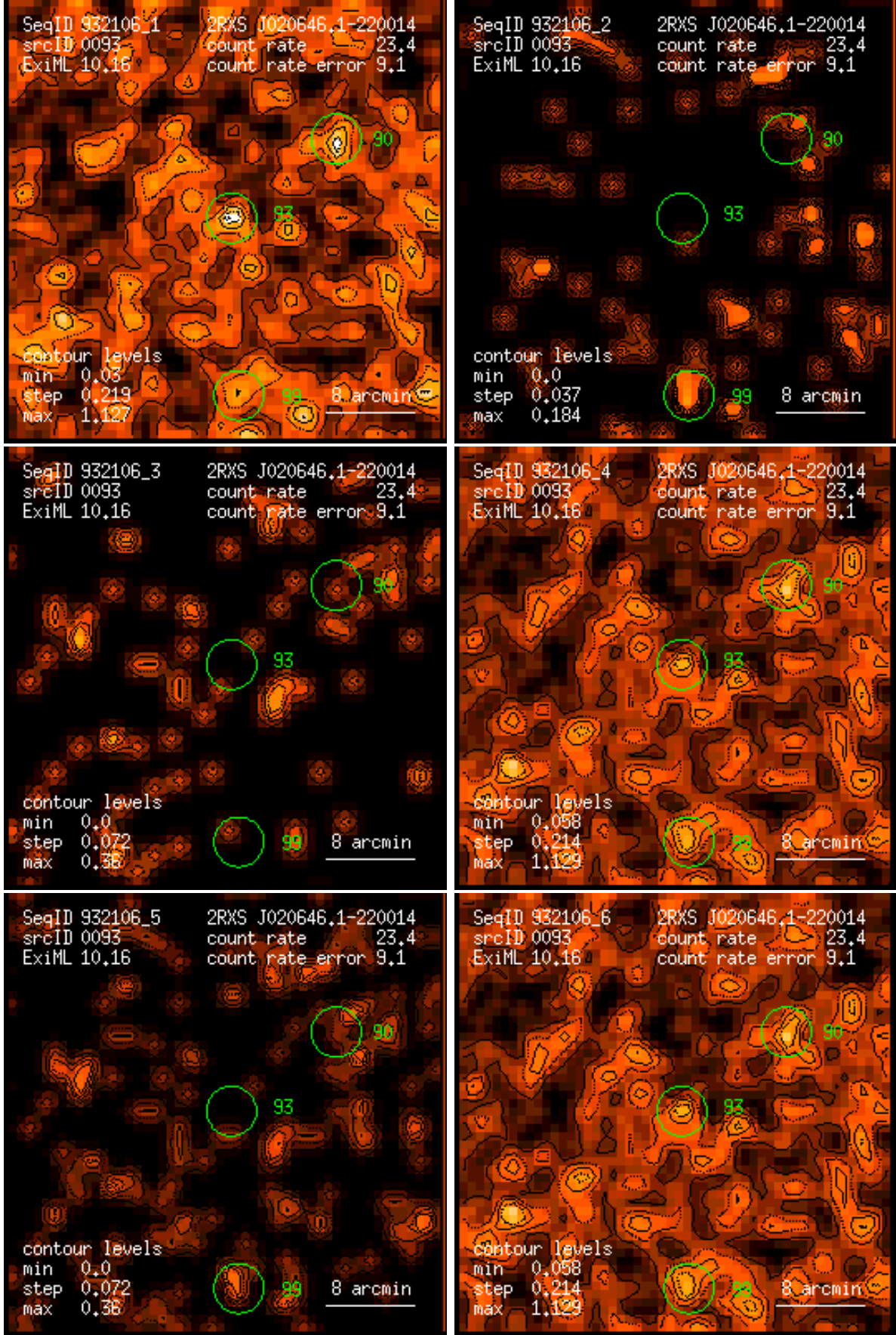
Figure 93: RASS 932106: detection 0093: band rate images, Gaussian filter: (1) PSPC channels 11 – 41, (2) 52 – 90, (3) 91 – 201, (4) 11 – 235, (5) 52 – 201, (6) 11 – 201. Broad band rates in counts/ks. Band rate contour levels in counts/ks/arcmin 2 .
