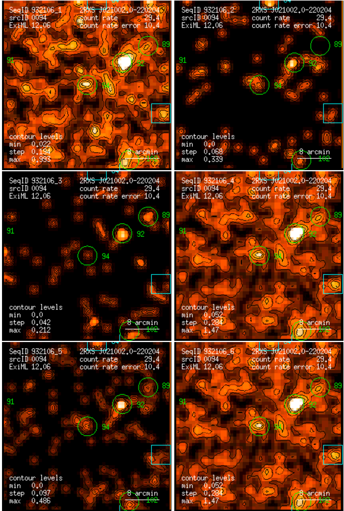
Figure 94: RASS 932106: detection 0094: band rate images, Gaussian filter: (1) PSPC channels 11 – 41, (2) 52 – 90, (3) 91 – 201, (4) 11 – 235, (5) 52 – 201, (6) 11 – 201. Broad band rates in counts/ks. Band rate contour levels in counts/ks/arcmin 2 .
