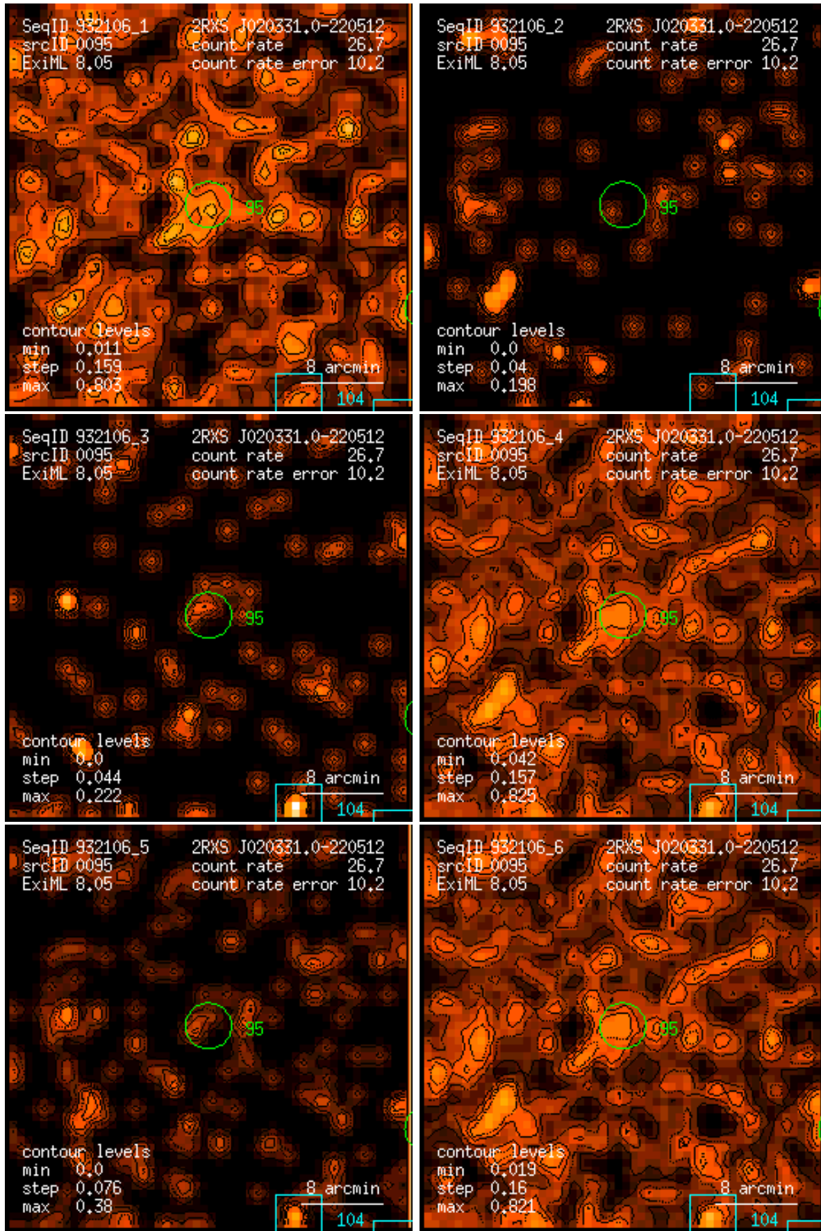
Figure 95: RASS 932106: detection 0095: band rate images, Gaussian filter: (1) PSPC channels 11 – 41, (2) 52 – 90, (3) 91 – 201, (4) 11 – 235, (5) 52 – 201, (6) 11 – 201. Broad band rates in counts/ks. Band rate contour levels in counts/ks/arcmin 2 .
