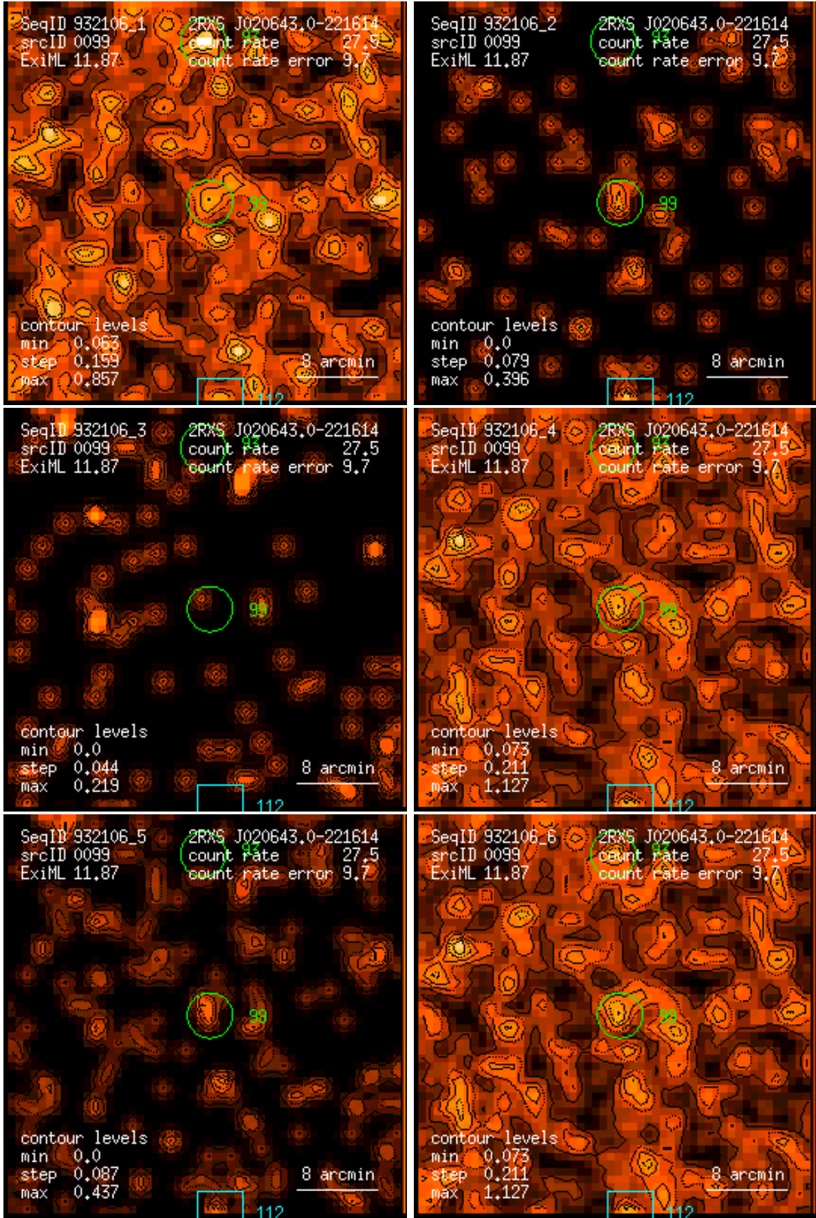
Figure 99: RASS 932106: detection 0099: band rate images, Gaussian filter: (1) PSPC channels 11 – 41, (2) 52 – 90, (3) 91 – 201, (4) 11 – 235, (5) 52 – 201, (6) 11 – 201. Broad band rates in counts/ks. Band rate contour levels in counts/ks/arcmin 2 .
