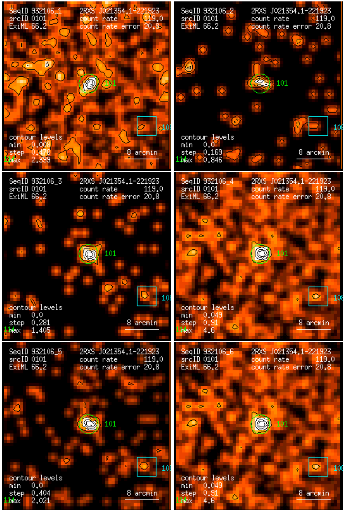
Figure 101: RASS 932106: detection 0101: band rate images, Gaussian filter: (1) PSPC channels 11 – 41, (2) 52 – 90, (3) 91 – 201, (4) 11 – 235, (5) 52 – 201, (6) 11 – 201. Broad band rates in counts/ks. Band rate contour levels in counts/ks/arcmin 2 .
