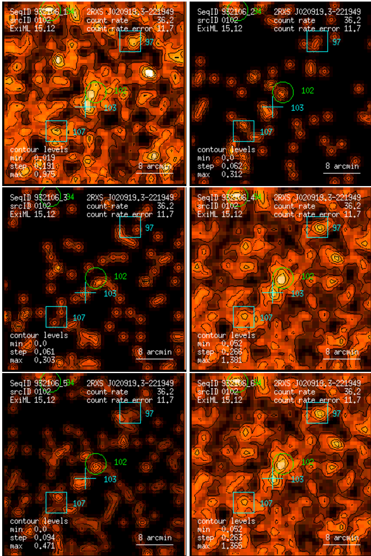
Figure 102: RASS 932106: detection 0102: band rate images, Gaussian filter: (1) PSPC channels 11 – 41, (2) 52 – 90, (3) 91 – 201, (4) 11 – 235, (5) 52 – 201, (6) 11 – 201. Broad band rates in counts/ks. Band rate contour levels in counts/ks/arcmin 2 .
