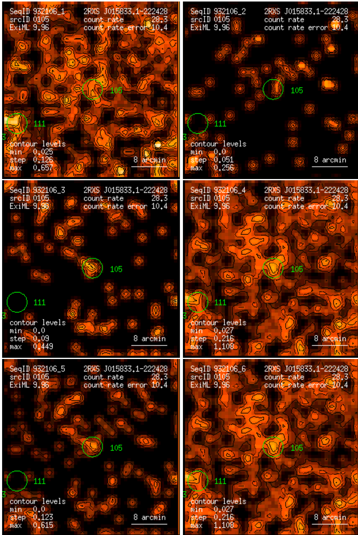
Figure 105: RASS 932106: detection 0105: band rate images, Gaussian filter: (1) PSPC channels 11 – 41, (2) 52 – 90, (3) 91 – 201, (4) 11 – 235, (5) 52 – 201, (6) 11 – 201. Broad band rates in counts/ks. Band rate contour levels in counts/ks/arcmin 2 .
