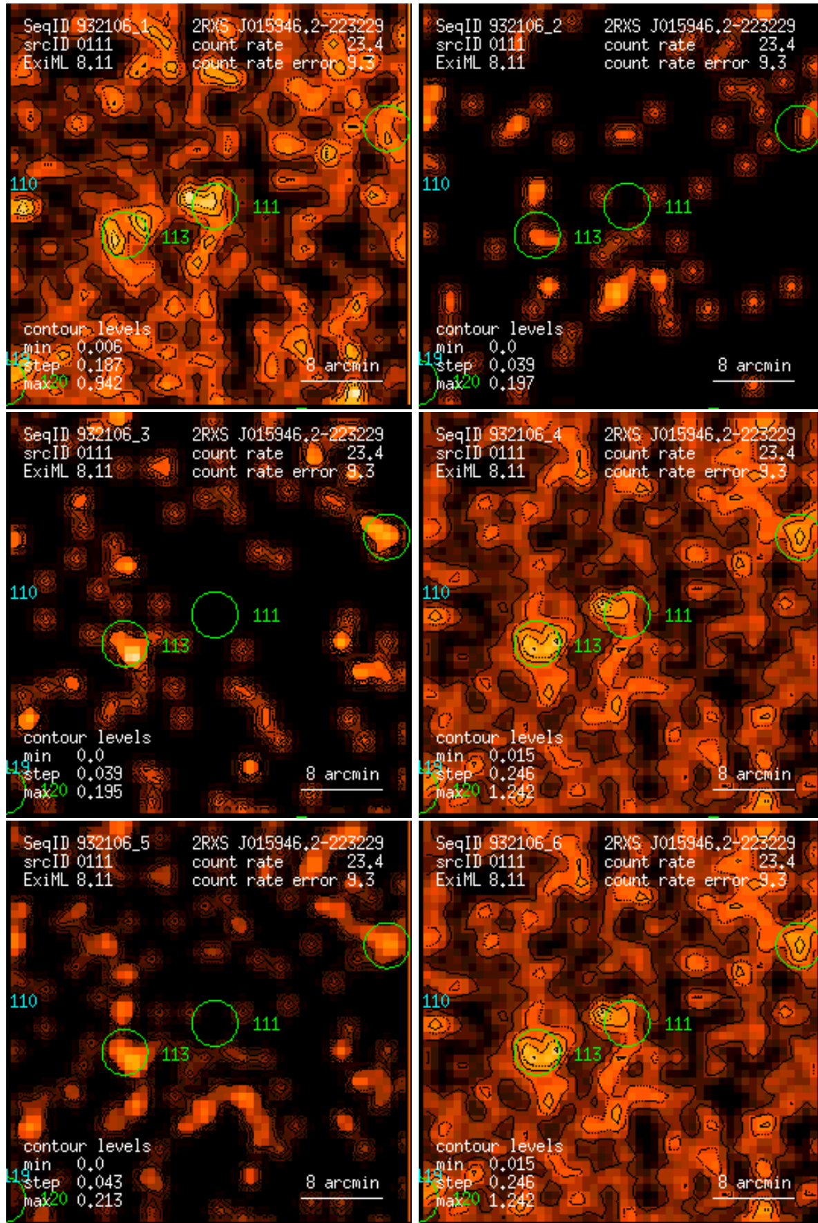
Figure 111: RASS 932106: detection 0111: band rate images, Gaussian filter: (1) PSPC channels 11 – 41, (2) 52 – 90, (3) 91 – 201, (4) 11 – 235, (5) 52 – 201, (6) 11 – 201. Broad band rates in counts/ks. Band rate contour levels in counts/ks/arcmin 2 .
