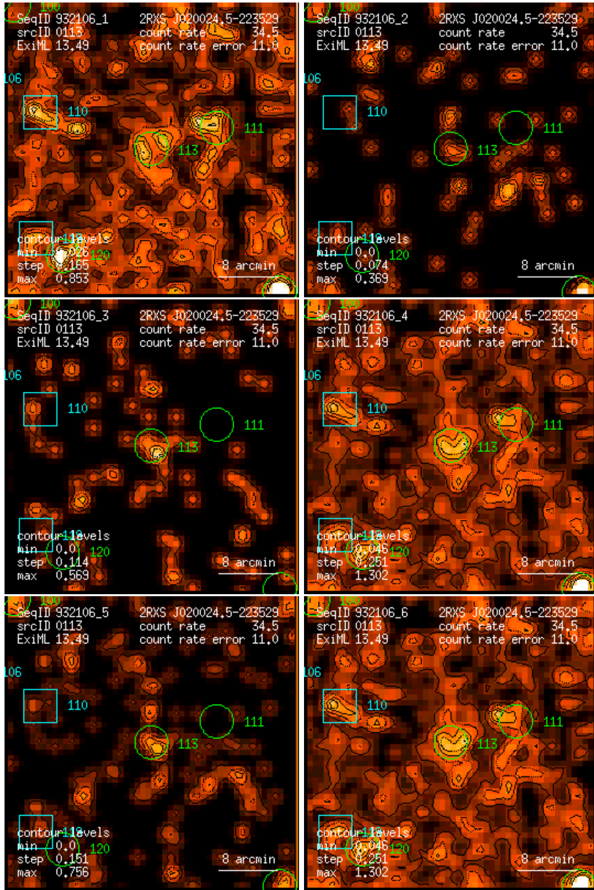
Figure 113: RASS 932106: detection 0113: band rate images, Gaussian filter: (1) PSPC channels 11 – 41, (2) 52 – 90, (3) 91 – 201, (4) 11 – 235, (5) 52 – 201, (6) 11 – 201. Broad band rates in counts/ks. Band rate contour levels in counts/ks/arcmin 2 .
