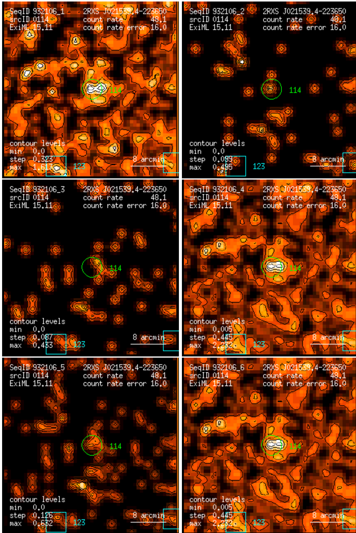
Figure 114: RASS 932106: detection 0114: band rate images, Gaussian filter: (1) PSPC channels 11 – 41, (2) 52 – 90, (3) 91 – 201, (4) 11 – 235, (5) 52 – 201, (6) 11 – 201. Broad band rates in counts/ks. Band rate contour levels in counts/ks/arcmin 2 .
