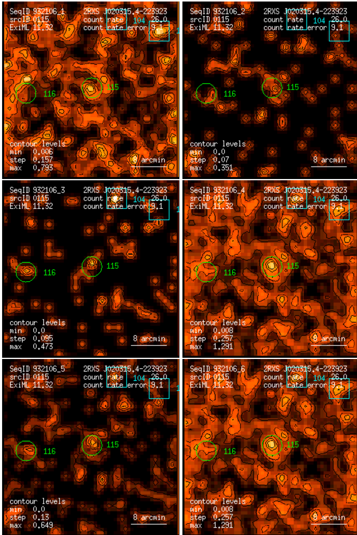
Figure 115: RASS 932106: detection 0115: band rate images, Gaussian filter: (1) PSPC channels 11 – 41, (2) 52 – 90, (3) 91 – 201, (4) 11 – 235, (5) 52 – 201, (6) 11 – 201. Broad band rates in counts/ks. Band rate contour levels in counts/ks/arcmin 2 .
