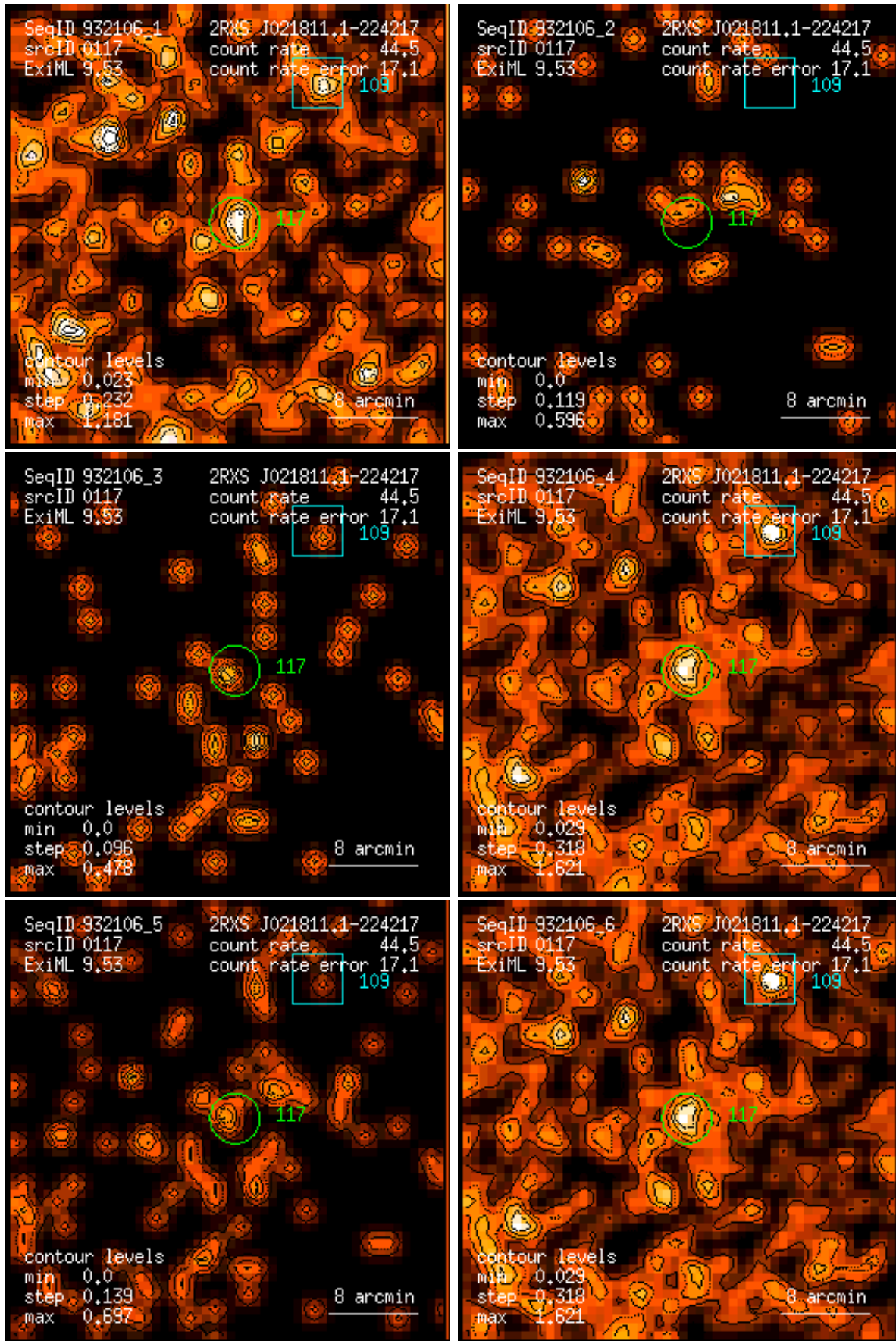
Figure 117: RASS 932106: detection 0117: band rate images, Gaussian filter: (1) PSPC channels 11 – 41, (2) 52 – 90, (3) 91 – 201, (4) 11 – 235, (5) 52 – 201, (6) 11 – 201. Broad band rates in counts/ks. Band rate contour levels in counts/ks/arcmin 2 .
