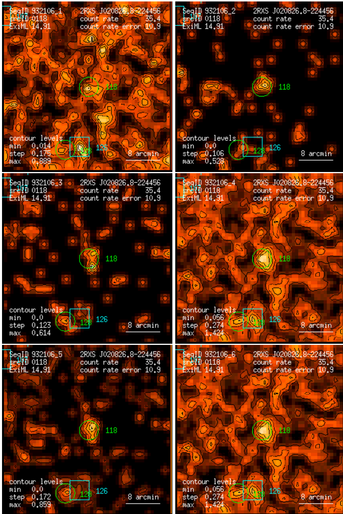
Figure 118: RASS 932106: detection 0118: band rate images, Gaussian filter: (1) PSPC channels 11 – 41, (2) 52 – 90, (3) 91 – 201, (4) 11 – 235, (5) 52 – 201, (6) 11 – 201. Broad band rates in counts/ks. Band rate contour levels in counts/ks/arcmin 2 .
