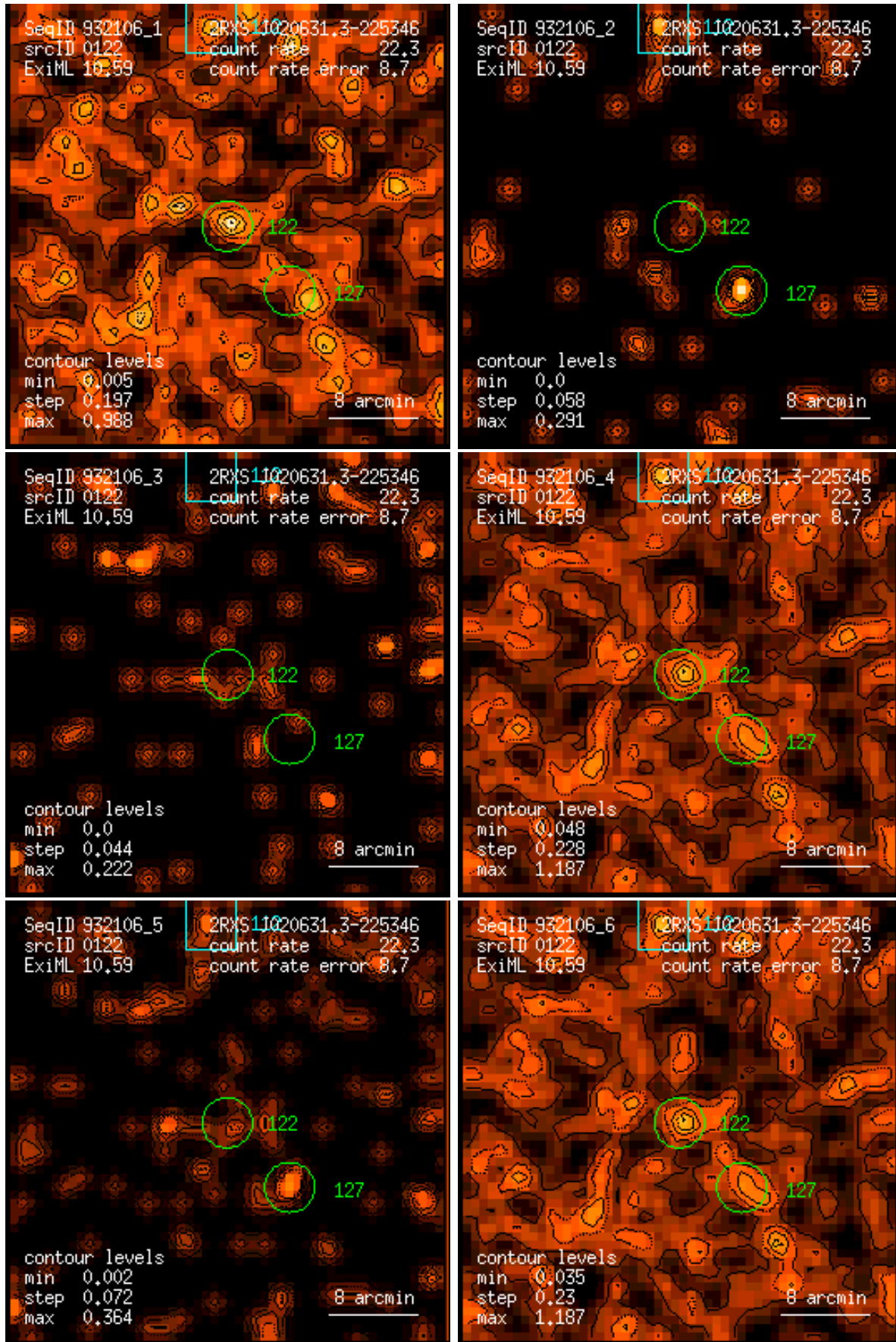
Figure 122: RASS 932106: detection 0122: band rate images, Gaussian filter: (1) PSPC channels 11 – 41, (2) 52 – 90, (3) 91 – 201, (4) 11 – 235, (5) 52 – 201, (6) 11 – 201. Broad band rates in counts/ks. Band rate contour levels in counts/ks/arcmin 2 .
