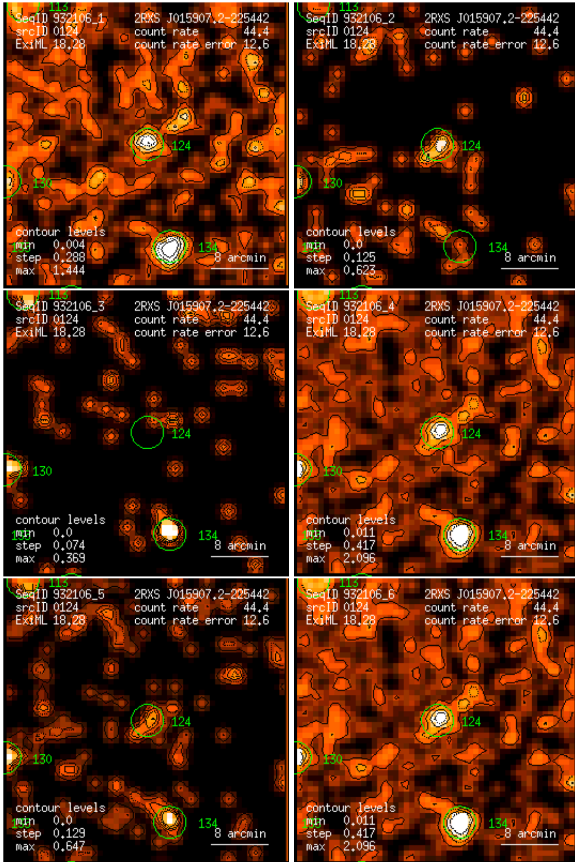
Figure 124: RASS 932106: detection 0124: band rate images, Gaussian filter: (1) PSPC channels 11 – 41, (2) 52 – 90, (3) 91 – 201, (4) 11 – 235, (5) 52 – 201, (6) 11 – 201. Broad band rates in counts/ks. Band rate contour levels in counts/ks/arcmin 2 .
