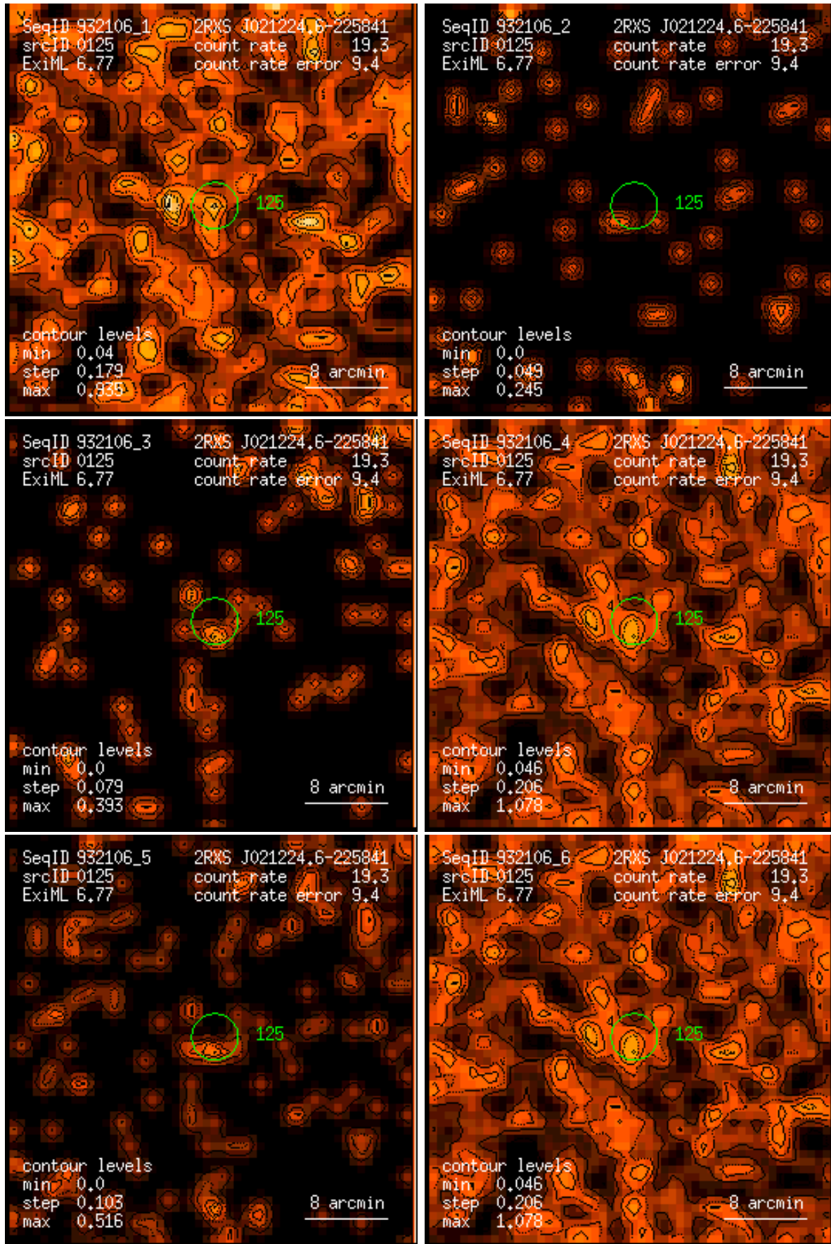
Figure 125: RASS 932106: detection 0125: band rate images, Gaussian filter: (1) PSPC channels 11 – 41, (2) 52 – 90, (3) 91 – 201, (4) 11 – 235, (5) 52 – 201, (6) 11 – 201. Broad band rates in counts/ks. Band rate contour levels in counts/ks/arcmin 2 .
