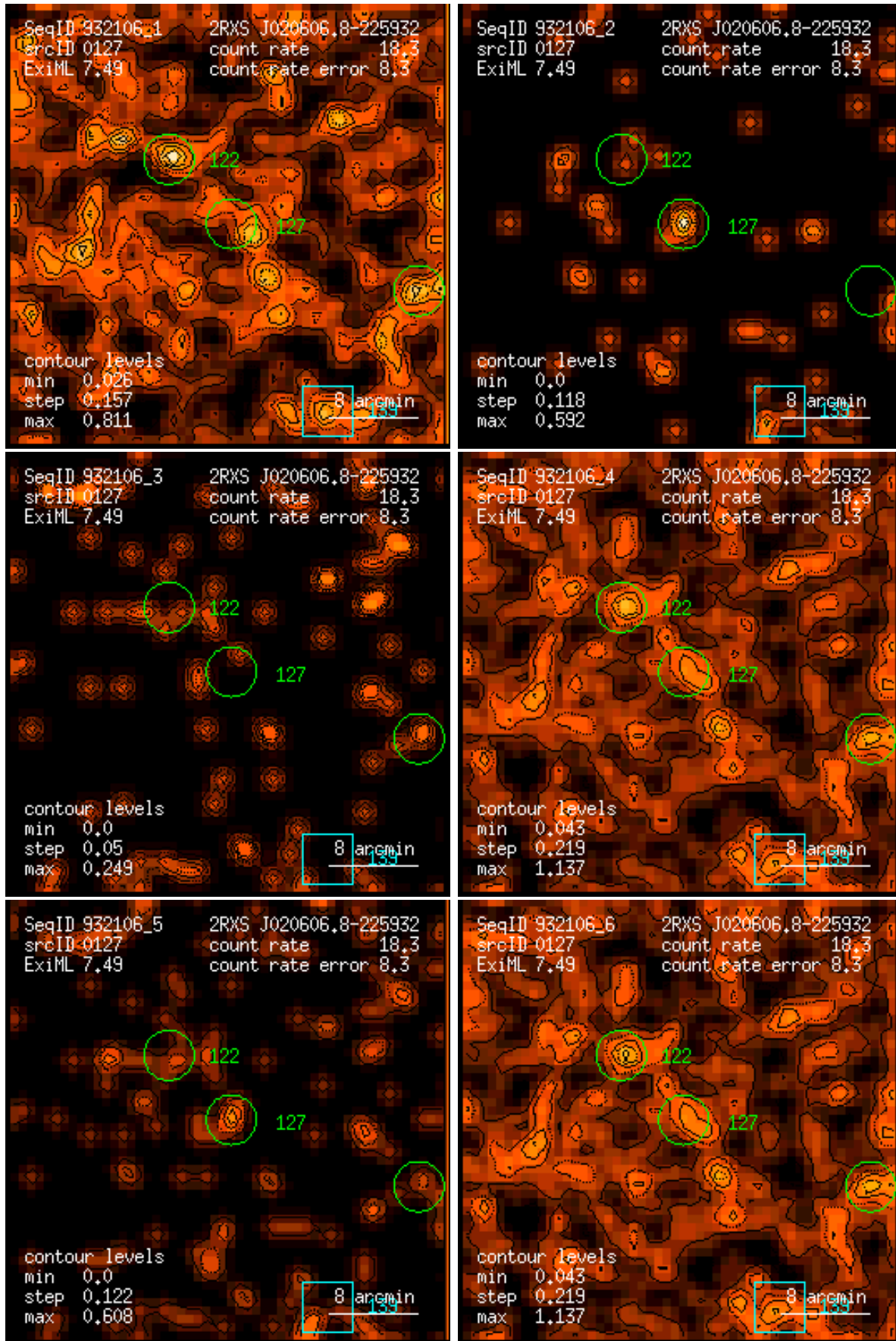
Figure 127: RASS 932106: detection 0127: band rate images, Gaussian filter: (1) PSPC channels 11 – 41, (2) 52 – 90, (3) 91 – 201, (4) 11 – 235, (5) 52 – 201, (6) 11 – 201. Broad band rates in counts/ks. Band rate contour levels in counts/ks/arcmin 2 .
