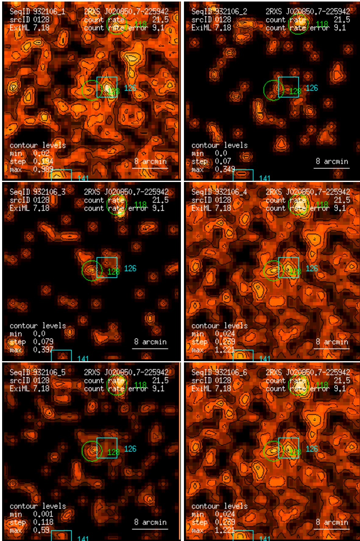
Figure 128: RASS 932106: detection 0128: band rate images, Gaussian filter: (1) PSPC channels 11 – 41, (2) 52 – 90, (3) 91 – 201, (4) 11 – 235, (5) 52 – 201, (6) 11 – 201. Broad band rates in counts/ks. Band rate contour levels in counts/ks/arcmin 2 .
