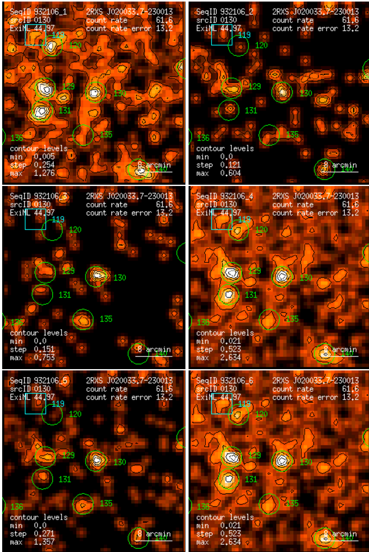
Figure 130: RASS 932106: detection 0130: band rate images, Gaussian filter: (1) PSPC channels 11 – 41, (2) 52 – 90, (3) 91 – 201, (4) 11 – 235, (5) 52 – 201, (6) 11 – 201. Broad band rates in counts/ks. Band rate contour levels in counts/ks/arcmin 2 .
