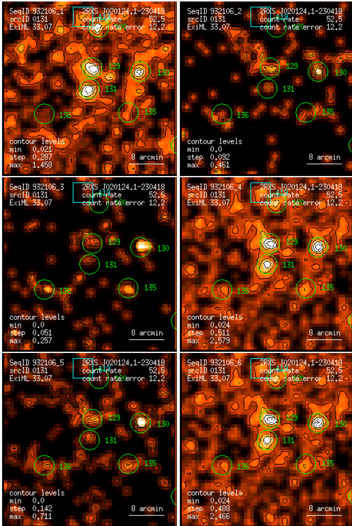
Figure 131: RASS 932106: detection 0131: band rate images, Gaussian filter: (1) PSPC channels 11 – 41, (2) 52 – 90, (3) 91 – 201, (4) 11 – 235, (5) 52 – 201, (6) 11 – 201. Broad band rates in counts/ks. Band rate contour levels in counts/ks/arcmin 2 .
