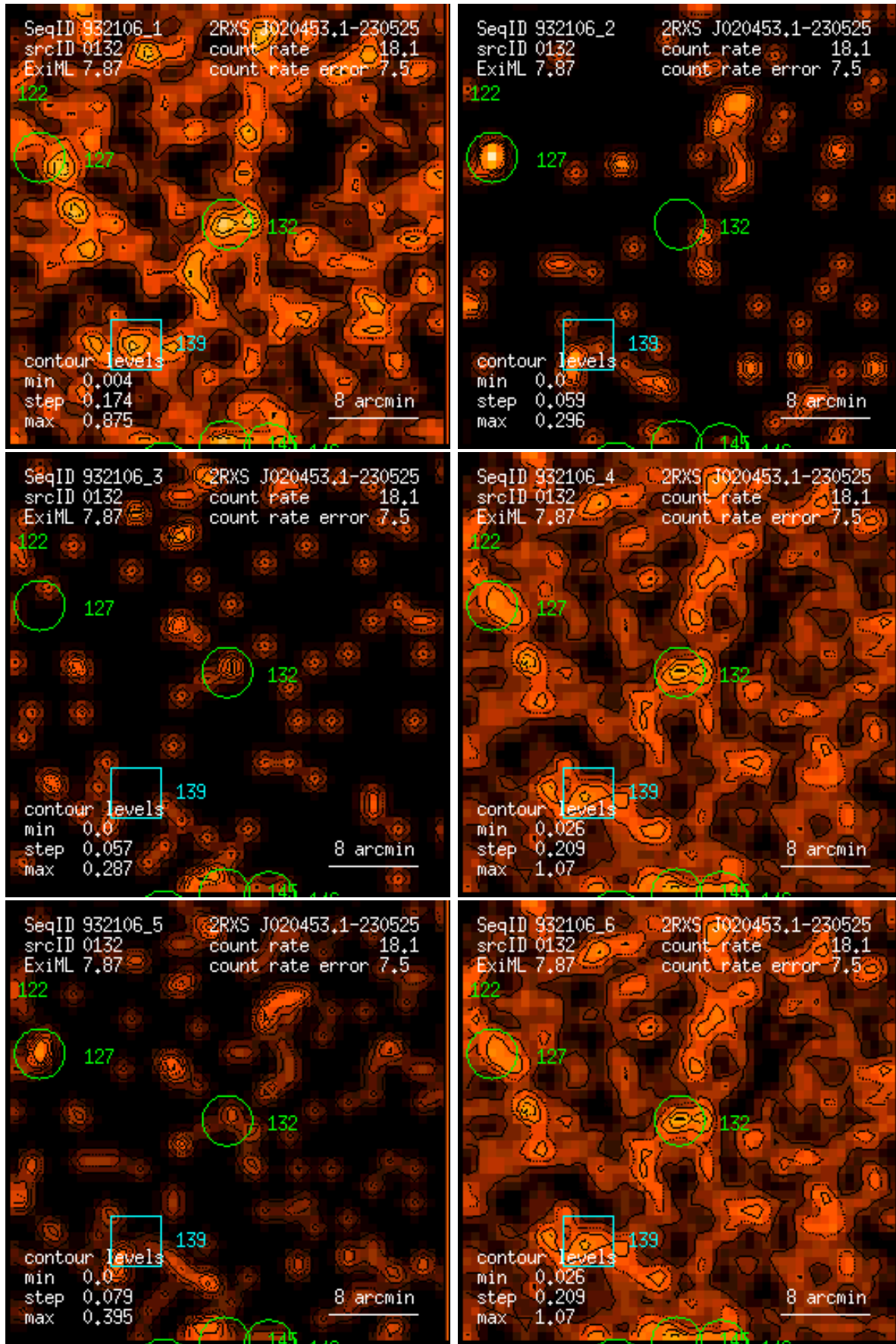
Figure 132: RASS 932106: detection 0132: band rate images, Gaussian filter: (1) PSPC channels 11 – 41, (2) 52 – 90, (3) 91 – 201, (4) 11 – 235, (5) 52 – 201, (6) 11 – 201. Broad band rates in counts/ks. Band rate contour levels in counts/ks/arcmin 2 .
