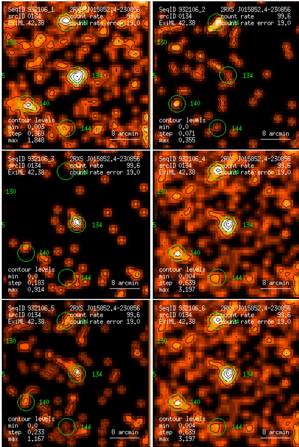
Figure 134: RASS 932106: detection 0134: band rate images, Gaussian filter: (1) PSPC channels 11 – 41, (2) 52 – 90, (3) 91 – 201, (4) 11 – 235, (5) 52 – 201, (6) 11 – 201. Broad band rates in counts/ks. Band rate contour levels in counts/ks/arcmin 2 .
