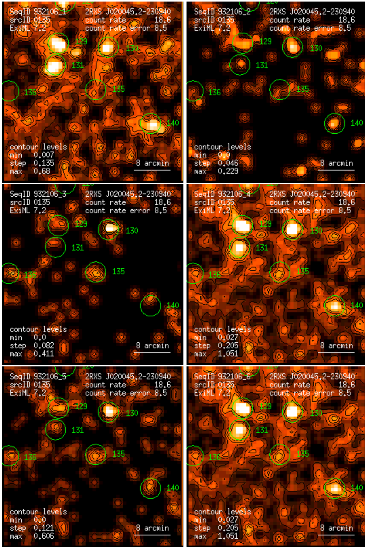
Figure 135: RASS 932106: detection 0135: band rate images, Gaussian filter: (1) PSPC channels 11 – 41, (2) 52 – 90, (3) 91 – 201, (4) 11 – 235, (5) 52 – 201, (6) 11 – 201. Broad band rates in counts/ks. Band rate contour levels in counts/ks/arcmin 2 .
