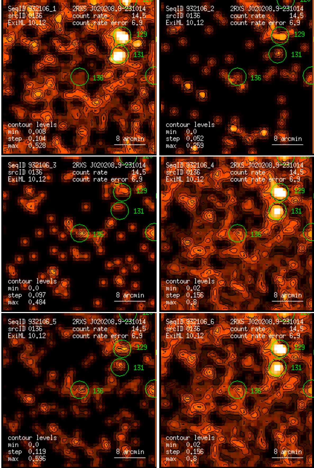
Figure 136: RASS 932106: detection 0136: band rate images, Gaussian filter: (1) PSPC channels 11 – 41, (2) 52 – 90, (3) 91 – 201, (4) 11 – 235, (5) 52 – 201, (6) 11 – 201. Broad band rates in counts/ks. Band rate contour levels in counts/ks/arcmin 2 .
