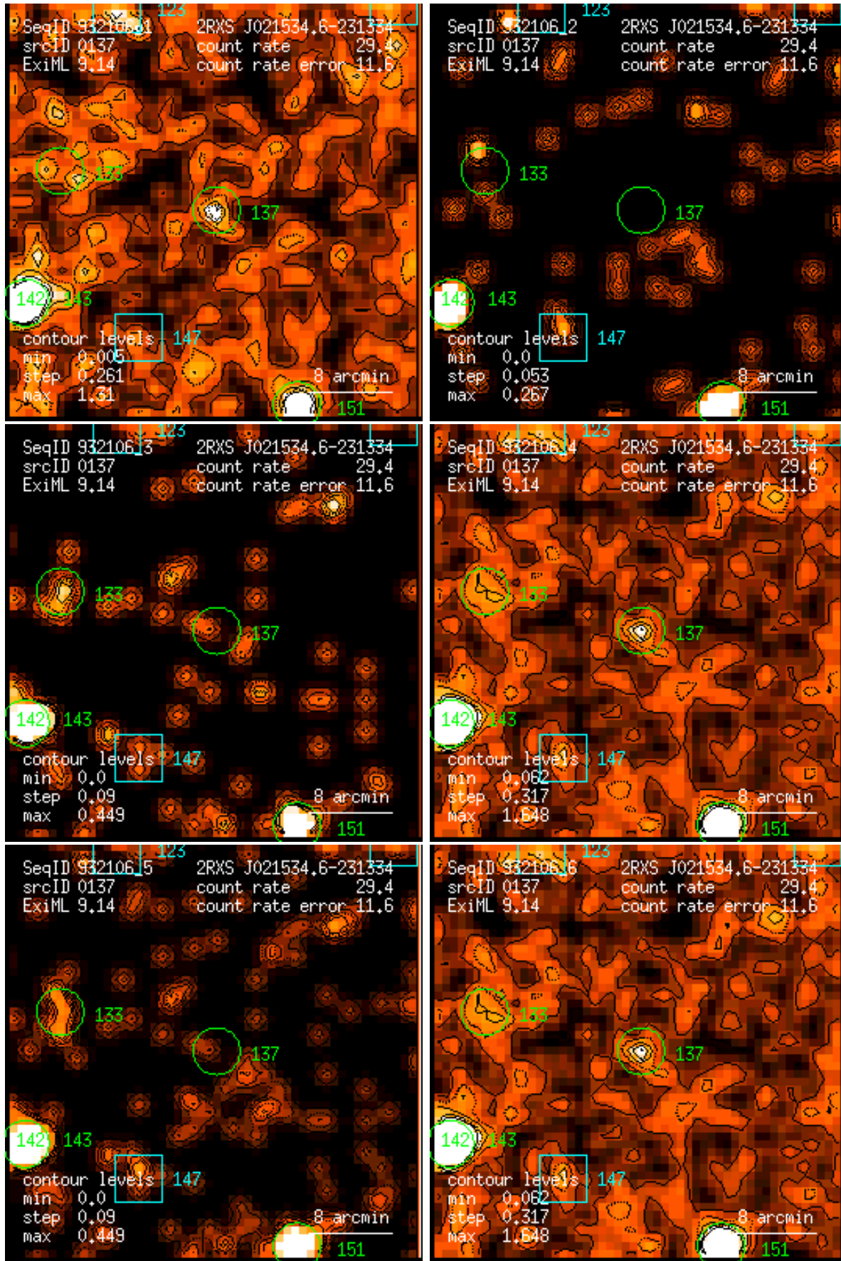
Figure 137: RASS 932106: detection 0137: band rate images, Gaussian filter: (1) PSPC channels 11 – 41, (2) 52 – 90, (3) 91 – 201, (4) 11 – 235, (5) 52 – 201, (6) 11 – 201. Broad band rates in counts/ks. Band rate contour levels in counts/ks/arcmin 2 .
