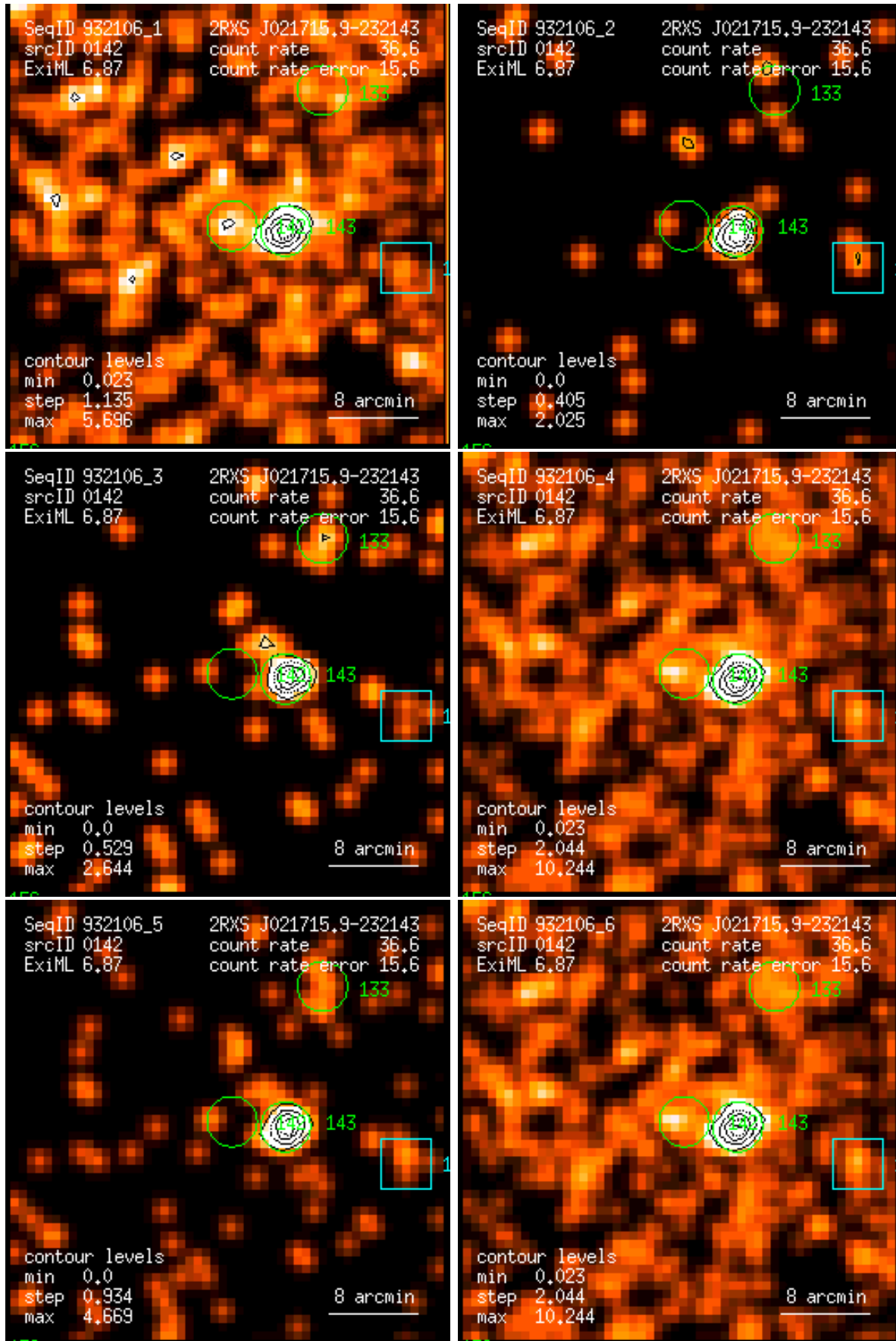
Figure 142: RASS 932106: detection 0142: band rate images, Gaussian filter: (1) PSPC channels 11 – 41, (2) 52 – 90, (3) 91 – 201, (4) 11 – 235, (5) 52 – 201, (6) 11 – 201. Broad band rates in counts/ks. Band rate contour levels in counts/ks/arcmin 2 .
