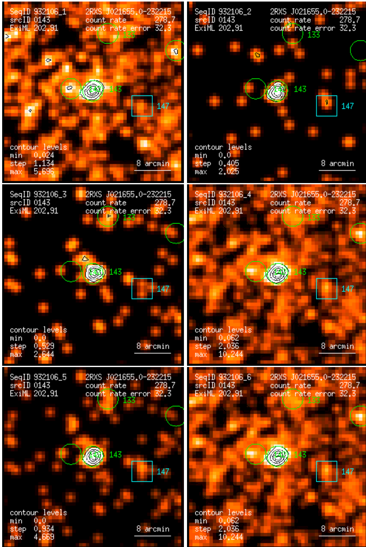
Figure 143: RASS 932106: detection 0143: band rate images, Gaussian filter: (1) PSPC channels 11 – 41, (2) 52 – 90, (3) 91 – 201, (4) 11 – 235, (5) 52 – 201, (6) 11 – 201. Broad band rates in counts/ks. Band rate contour levels in counts/ks/arcmin 2 .
