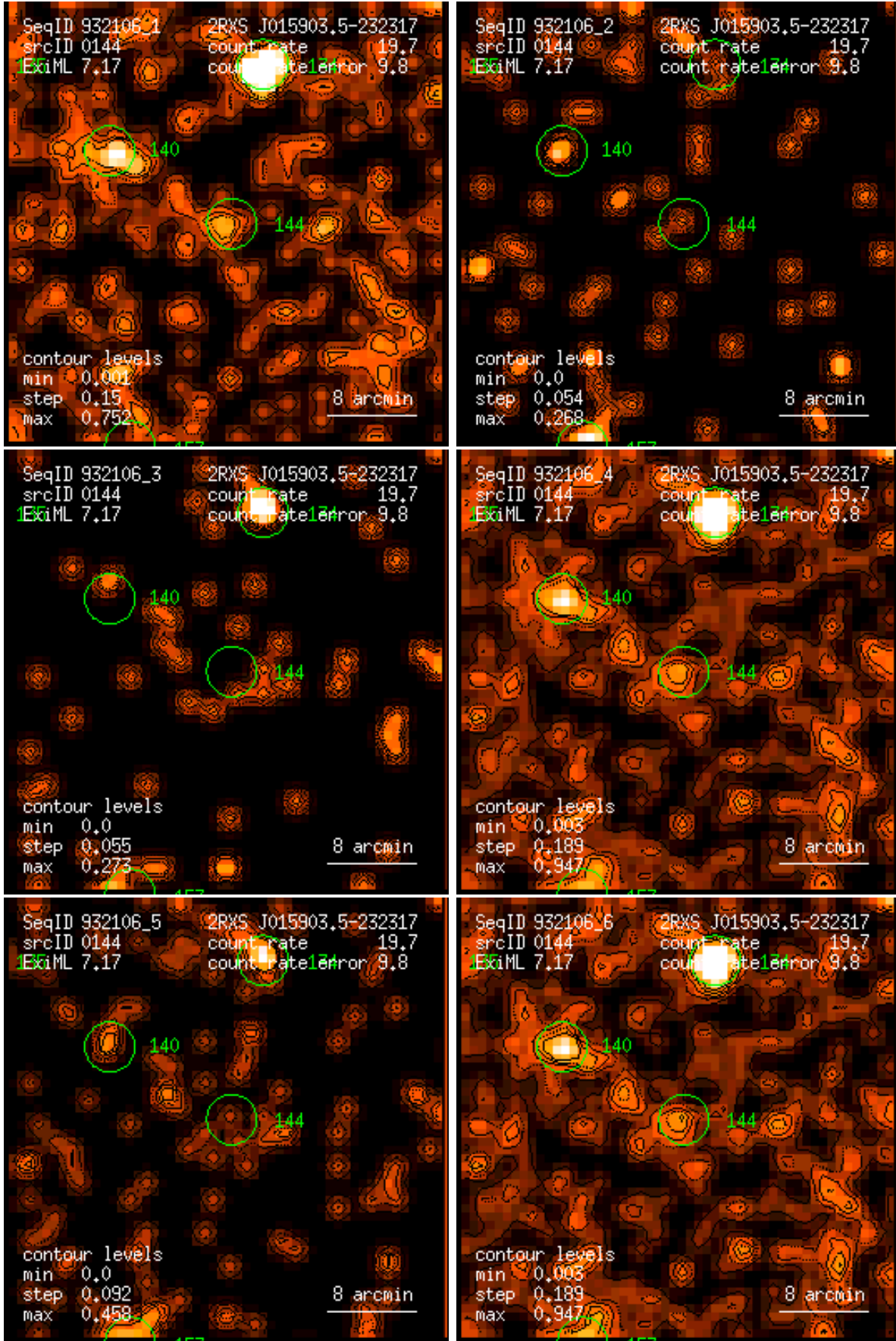
Figure 144: RASS 932106: detection 0144: band rate images, Gaussian filter: (1) PSPC channels 11 – 41, (2) 52 – 90, (3) 91 – 201, (4) 11 – 235, (5) 52 – 201, (6) 11 – 201. Broad band rates in counts/ks. Band rate contour levels in counts/ks/arcmin 2 .
