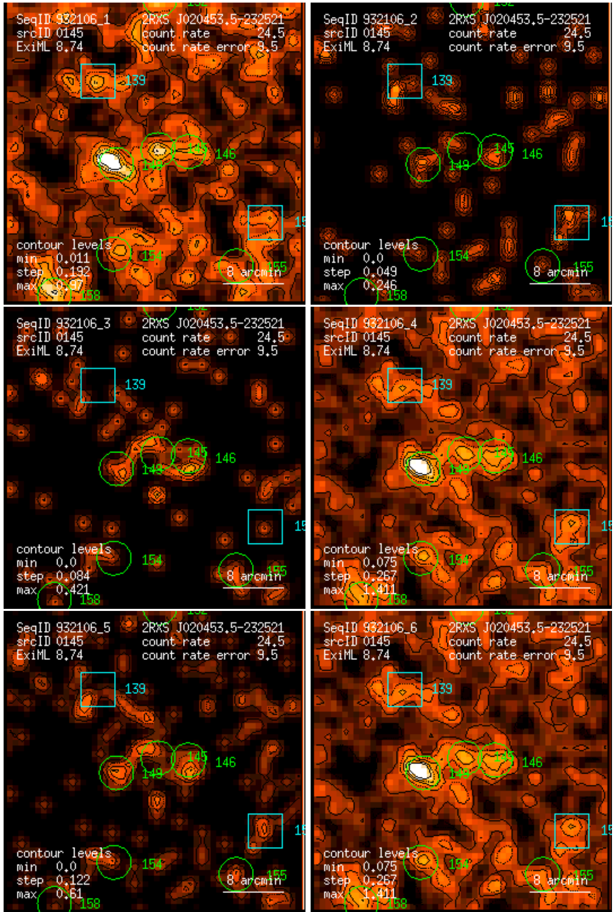
Figure 145: RASS 932106: detection 0145: band rate images, Gaussian filter: (1) PSPC channels 11 – 41, (2) 52 – 90, (3) 91 – 201, (4) 11 – 235, (5) 52 – 201, (6) 11 – 201. Broad band rates in counts/ks. Band rate contour levels in counts/ks/arcmin 2 .
