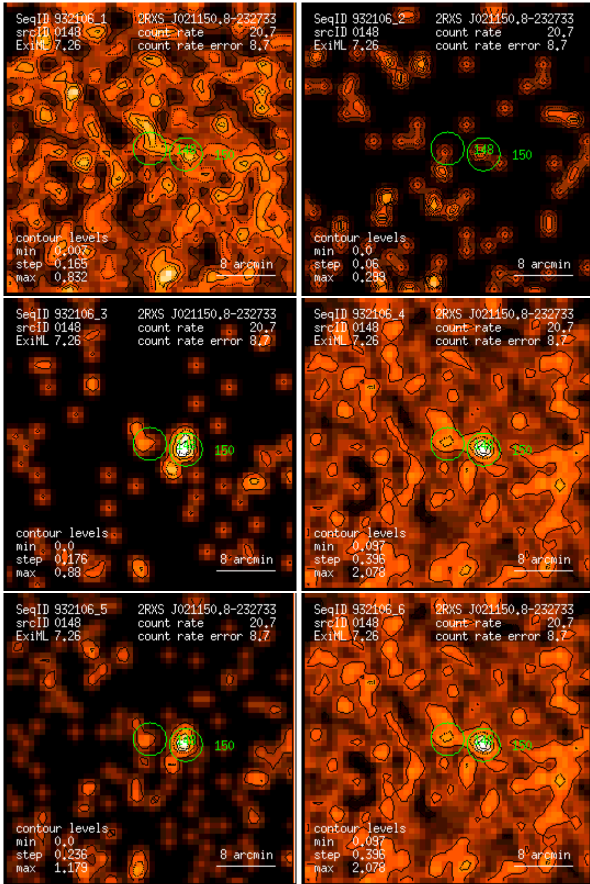
Figure 148: RASS 932106: detection 0148: band rate images, Gaussian filter: (1) PSPC channels 11 – 41, (2) 52 – 90, (3) 91 – 201, (4) 11 – 235, (5) 52 – 201, (6) 11 – 201. Broad band rates in counts/ks. Band rate contour levels in counts/ks/arcmin 2 .
