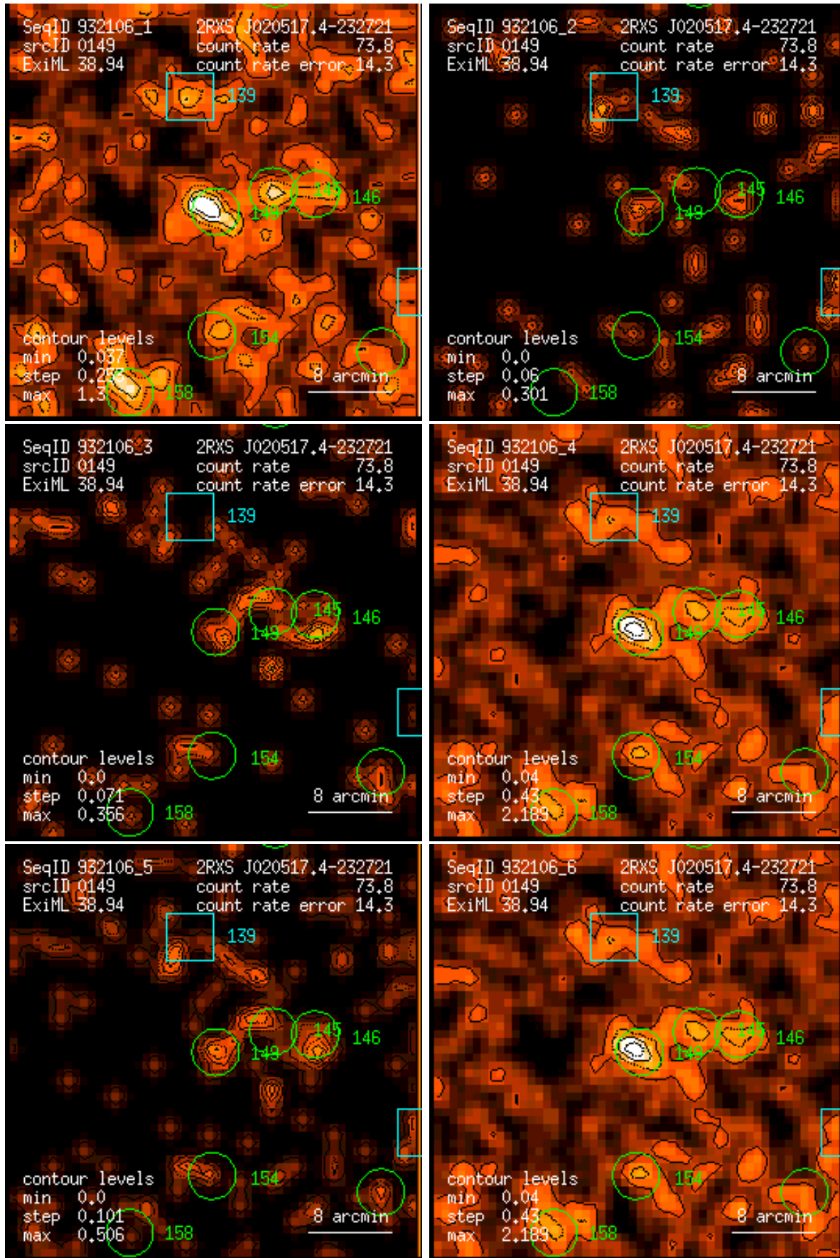
Figure 149: RASS 932106: detection 0149: band rate images, Gaussian filter: (1) PSPC channels 11 – 41, (2) 52 – 90, (3) 91 – 201, (4) 11 – 235, (5) 52 – 201, (6) 11 – 201. Broad band rates in counts/ks. Band rate contour levels in counts/ks/arcmin 2 .
