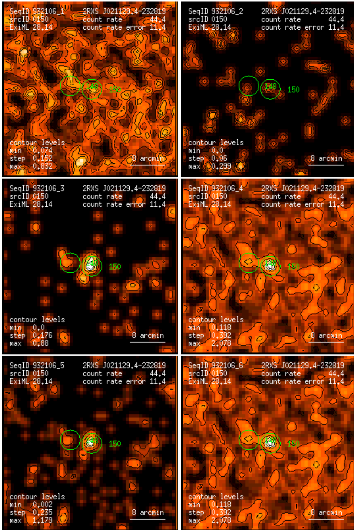
Figure 150: RASS 932106: detection 0150: band rate images, Gaussian filter: (1) PSPC channels 11 – 41, (2) 52 – 90, (3) 91 – 201, (4) 11 – 235, (5) 52 – 201, (6) 11 – 201. Broad band rates in counts/ks. Band rate contour levels in counts/ks/arcmin 2 .
