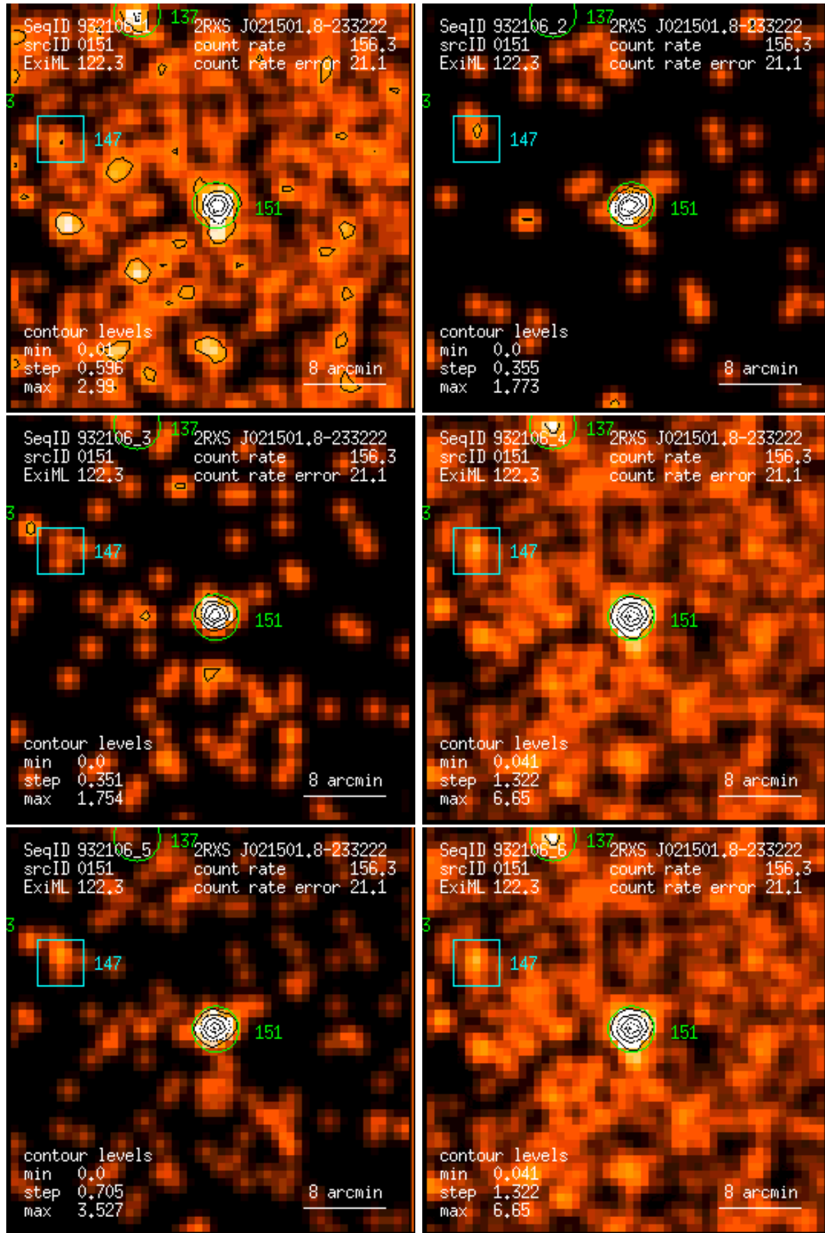
Figure 151: RASS 932106: detection 0151: band rate images, Gaussian filter: (1) PSPC channels 11 – 41, (2) 52 – 90, (3) 91 – 201, (4) 11 – 235, (5) 52 – 201, (6) 11 – 201. Broad band rates in counts/ks. Band rate contour levels in counts/ks/arcmin 2 .
