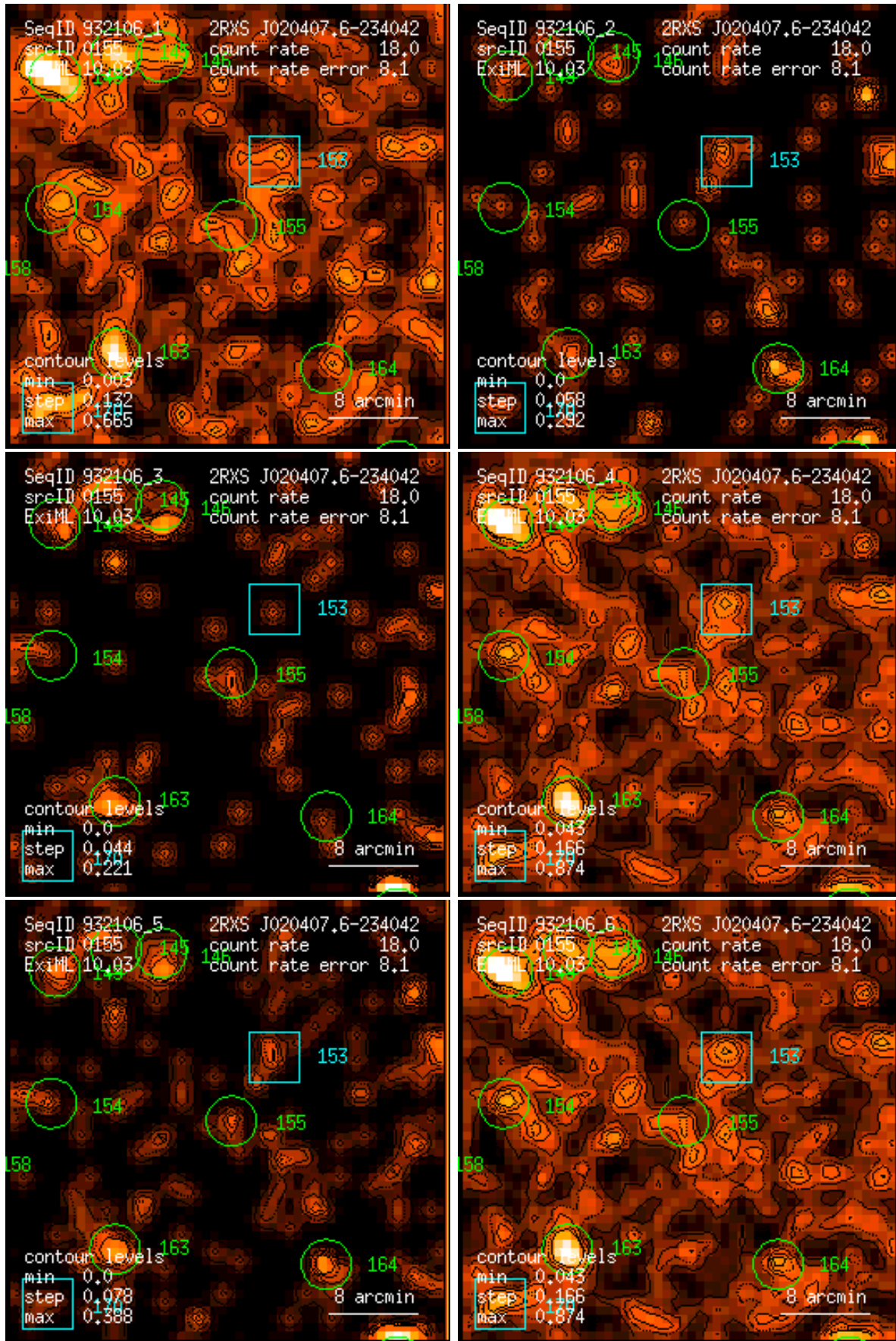
Figure 155: RASS 932106: detection 0155: band rate images, Gaussian filter: (1) PSPC channels 11 – 41, (2) 52 – 90, (3) 91 – 201, (4) 11 – 235, (5) 52 – 201, (6) 11 – 201. Broad band rates in counts/ks. Band rate contour levels in counts/ks/arcmin 2 .
