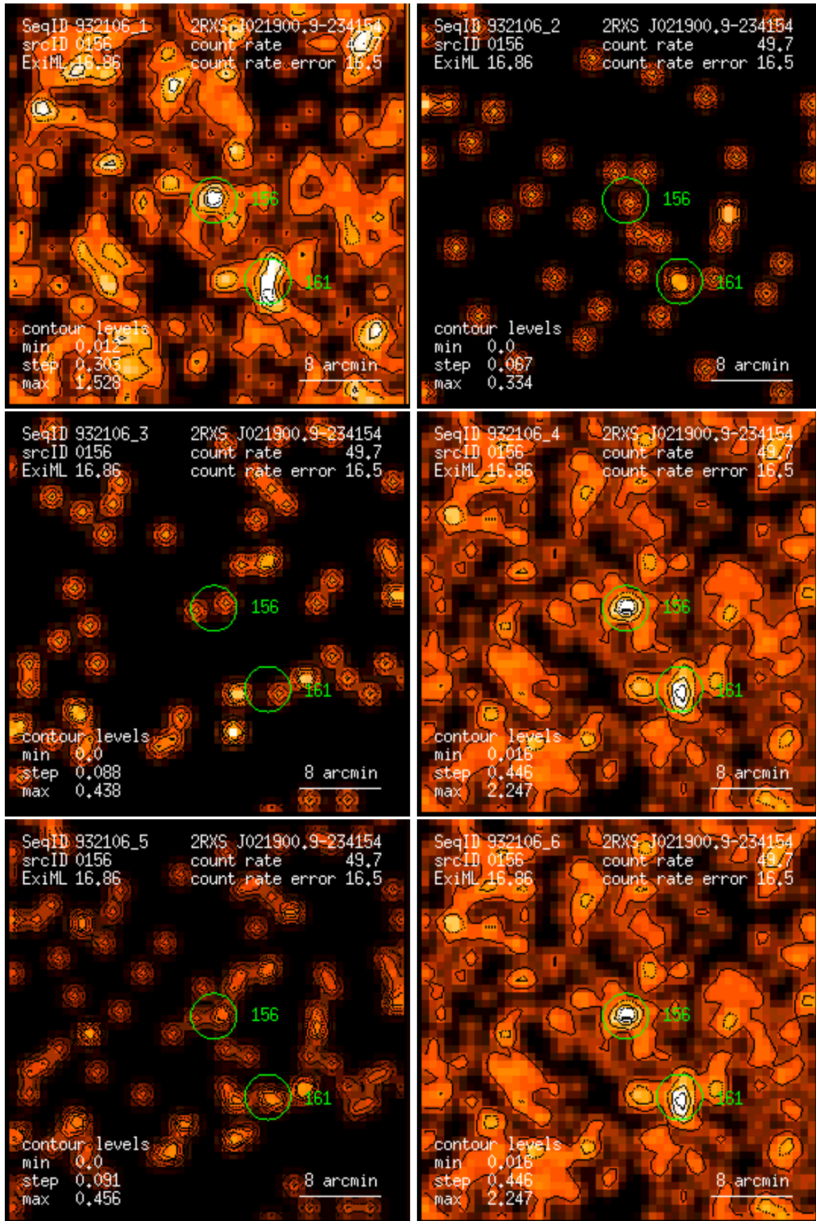
Figure 156: RASS 932106: detection 0156: band rate images, Gaussian filter: (1) PSPC channels 11 – 41, (2) 52 – 90, (3) 91 – 201, (4) 11 – 235, (5) 52 – 201, (6) 11 – 201. Broad band rates in counts/ks. Band rate contour levels in counts/ks/arcmin 2 .
