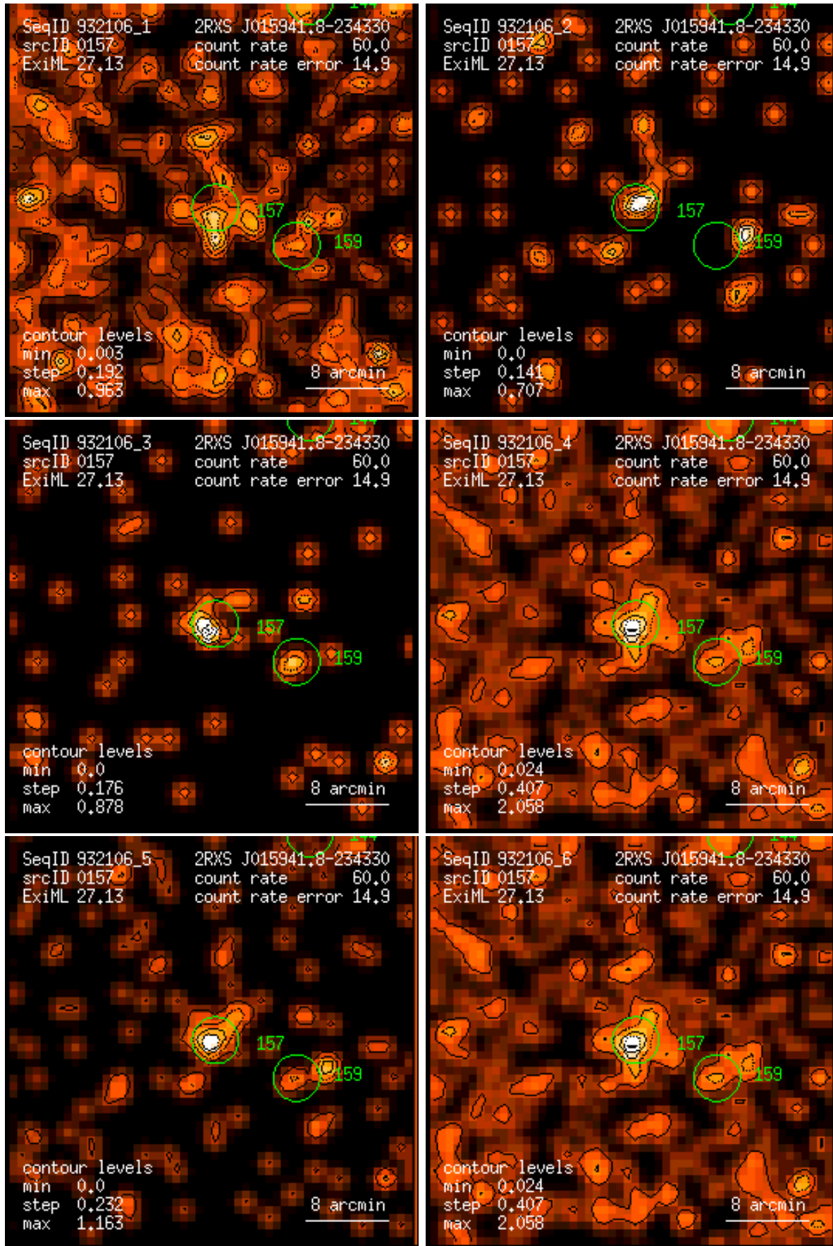
Figure 157: RASS 932106: detection 0157: band rate images, Gaussian filter: (1) PSPC channels 11 – 41, (2) 52 – 90, (3) 91 – 201, (4) 11 – 235, (5) 52 – 201, (6) 11 – 201. Broad band rates in counts/ks. Band rate contour levels in counts/ks/arcmin 2 .
