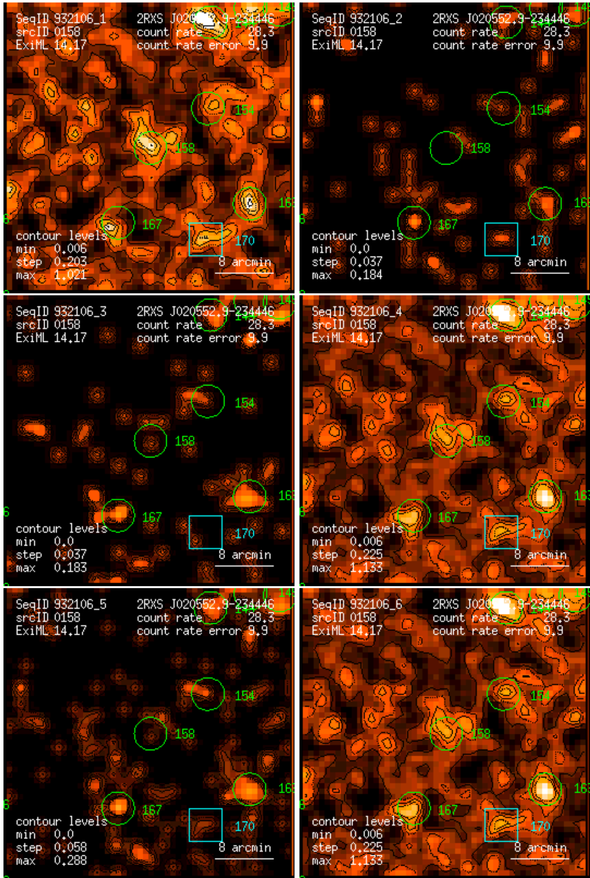
Figure 158: RASS 932106: detection 0158: band rate images, Gaussian filter: (1) PSPC channels 11 – 41, (2) 52 – 90, (3) 91 – 201, (4) 11 – 235, (5) 52 – 201, (6) 11 – 201. Broad band rates in counts/ks. Band rate contour levels in counts/ks/arcmin 2 .
