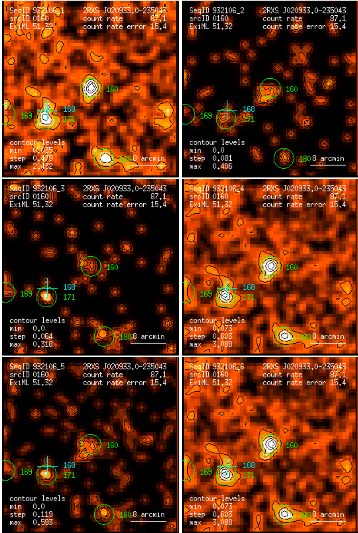
Figure 160: RASS 932106: detection 0160: band rate images, Gaussian filter: (1) PSPC channels 11 – 41, (2) 52 – 90, (3) 91 – 201, (4) 11 – 235, (5) 52 – 201, (6) 11 – 201. Broad band rates in counts/ks. Band rate contour levels in counts/ks/arcmin 2 .
