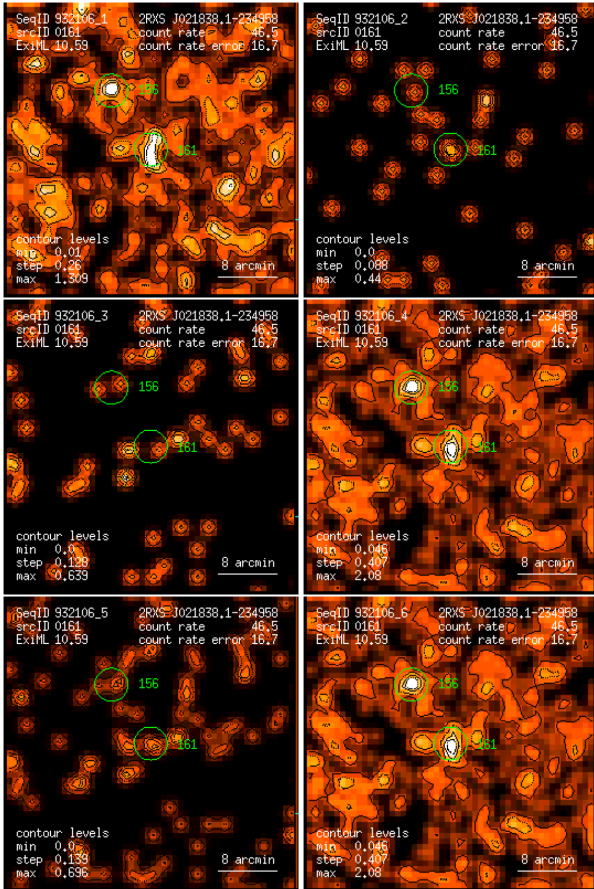
Figure 161: RASS 932106: detection 0161: band rate images, Gaussian filter: (1) PSPC channels 11 – 41, (2) 52 – 90, (3) 91 – 201, (4) 11 – 235, (5) 52 – 201, (6) 11 – 201. Broad band rates in counts/ks. Band rate contour levels in counts/ks/arcmin 2 .
