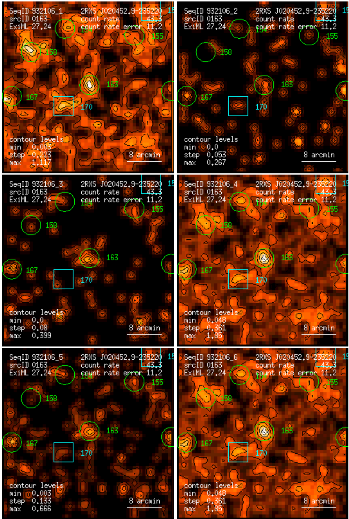
Figure 163: RASS 932106: detection 0163: band rate images, Gaussian filter: (1) PSPC channels 11 – 41, (2) 52 – 90, (3) 91 – 201, (4) 11 – 235, (5) 52 – 201, (6) 11 – 201. Broad band rates in counts/ks. Band rate contour levels in counts/ks/arcmin 2 .
