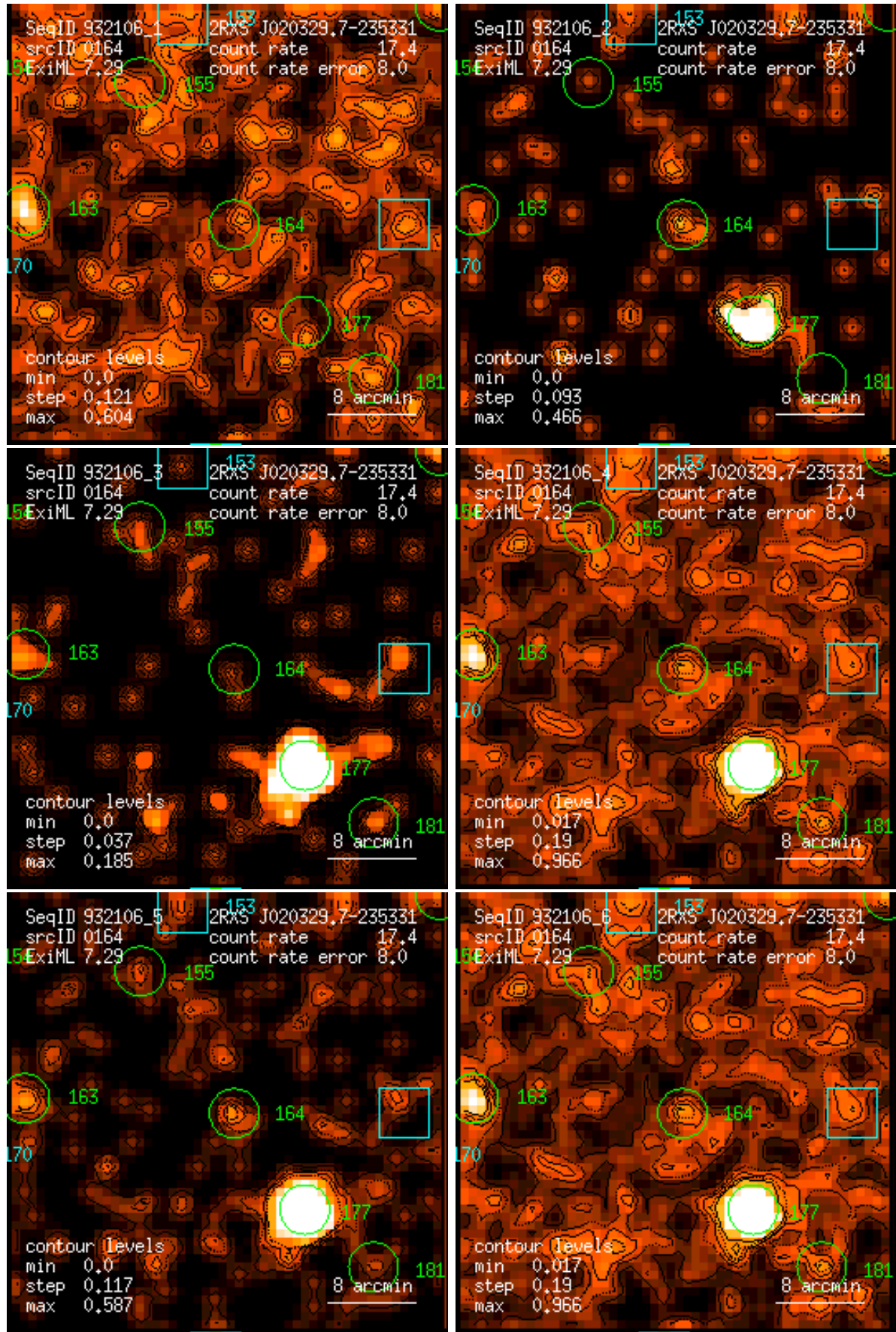
Figure 164: RASS 932106: detection 0164: band rate images, Gaussian filter: (1) PSPC channels 11 – 41, (2) 52 – 90, (3) 91 – 201, (4) 11 – 235, (5) 52 – 201, (6) 11 – 201. Broad band rates in counts/ks. Band rate contour levels in counts/ks/arcmin 2 .
